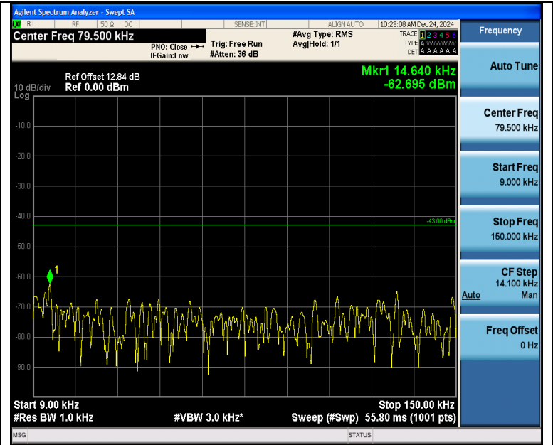
Band2_10MHz_16QAM_18650_1RB#49_0.009~0.15_0.009~0.15
