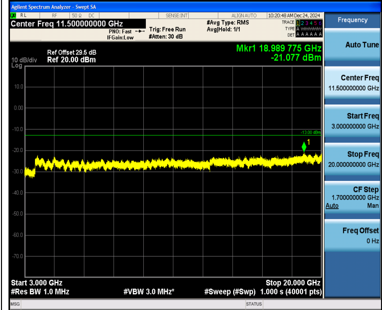
Band2_10MHz_QPSK_18650_1RB#0_3000~20000_3000~20000
