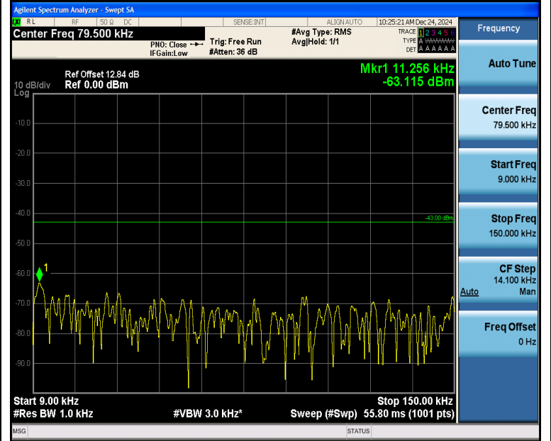
Band2_10MHz_16QAM_18900_1RB#0_0.009~0.15_0.009~0.15
