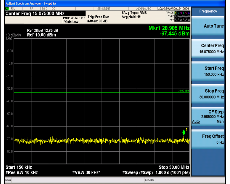
Band2_10MHz_QPSK_18650_1RB#0_0.15~30_0.15~30
