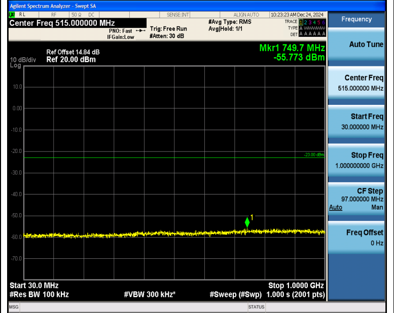
Band2_10MHz_16QAM_18650_1RB#49_30~1000_30~1000
