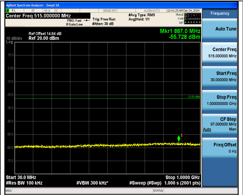
Band2_15MHz_QPSK_18675_1RB#74_30~1000_30~1000
