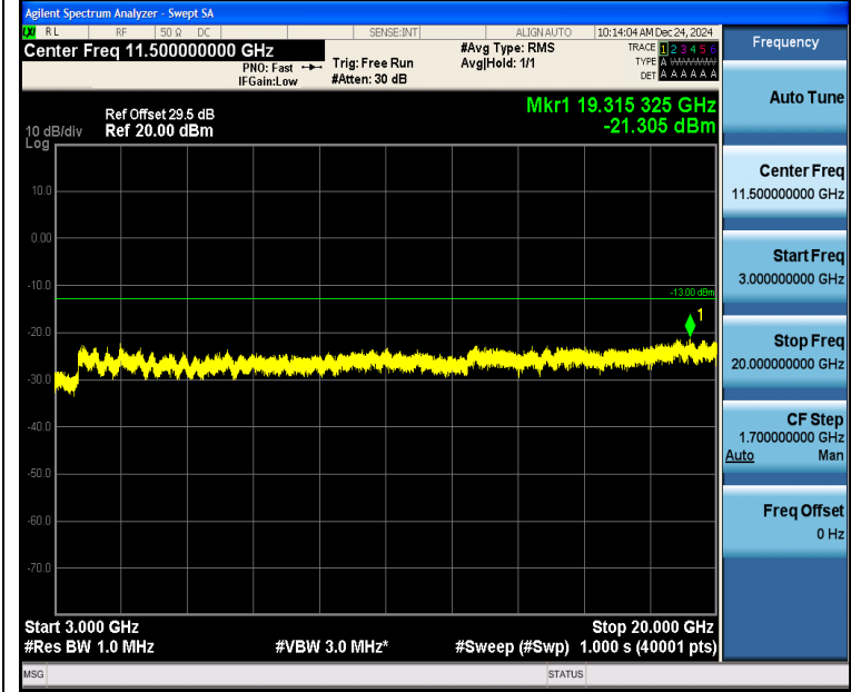
Band2_5MHz_QPSK_19175_1RB#24_3000~20000_3000~20000
