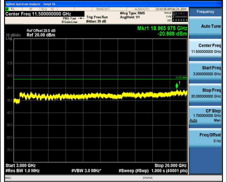
Band2_15MHz_QPSK_18675_1RB#74_3000~20000_3000~20000
