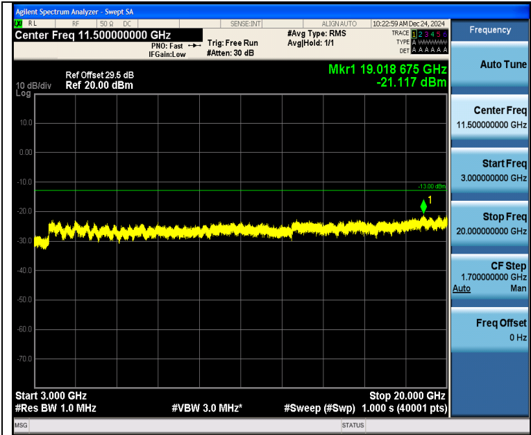
Band2_10MHz_QPSK_18650_1RB#49_3000~20000_3000~20000
