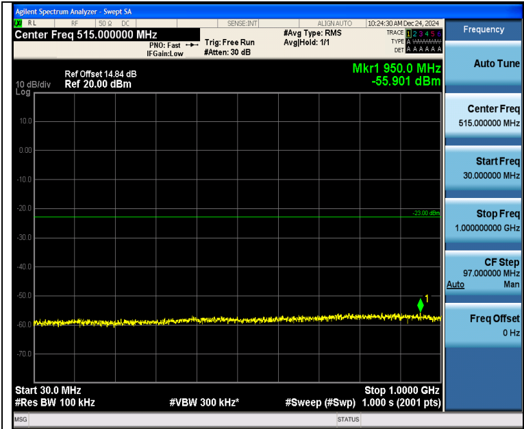
Band2_10MHz_QPSK_18900_1RB#0_30~1000_30~1000
