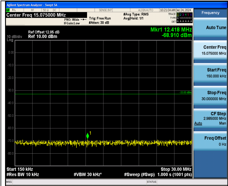
Band2_10MHz_16QAM_18650_1RB#0_0.15~30_0.15~30
