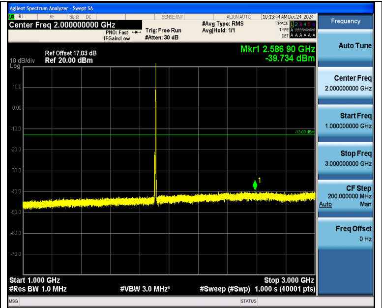
Band2_5MHz_QPSK_19175_1RB#24_1000~3000_1000~3000
