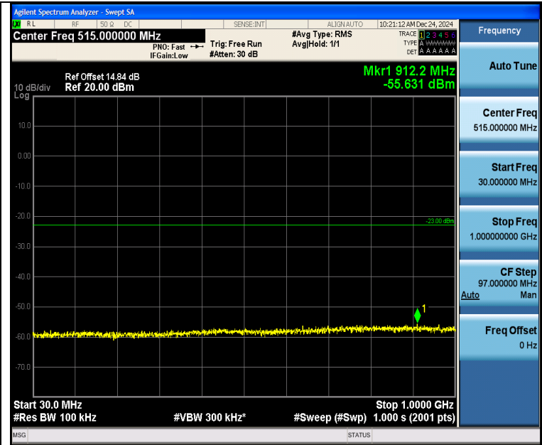
Band2_10MHz_16QAM_18650_1RB#0_30~1000_30~1000
