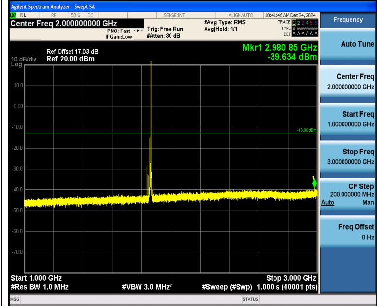
Band2_15MHz_QPSK_18675_1RB#74_1000~3000_1000~3000
