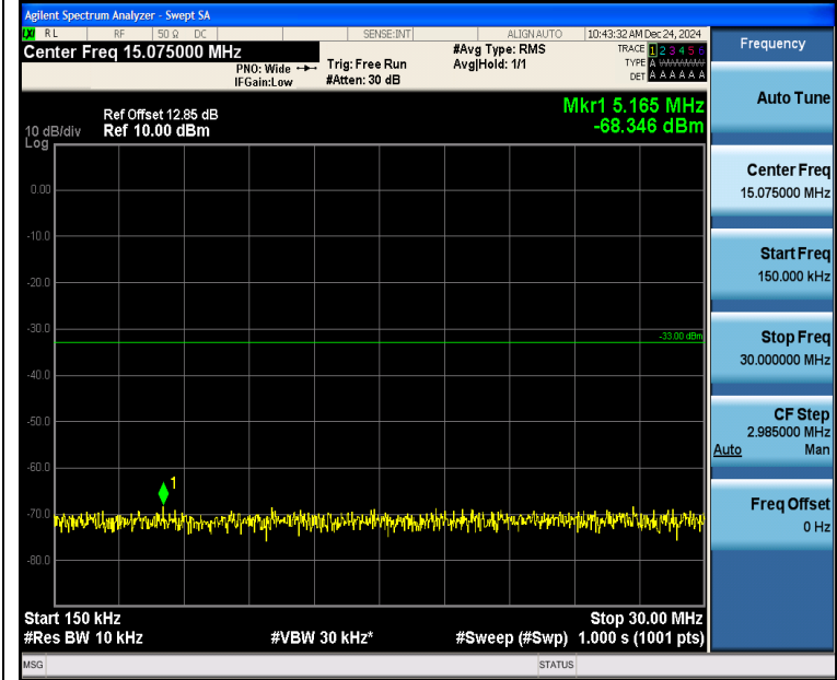
Band2_15MHz_QPSK_18900_1RB#0_0.15~30_0.15~30
