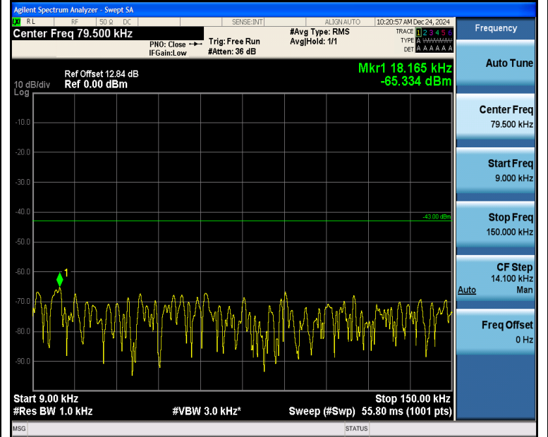
Band2_10MHz_16QAM_18650_1RB#0_0.009~0.15_0.009~0.15
