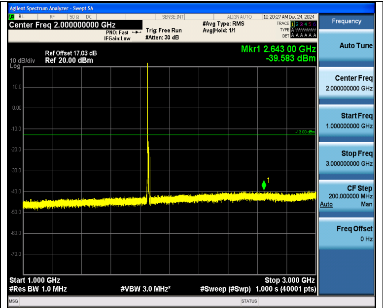
Band2_10MHz_QPSK_18650_1RB#0_1000~3000_1000~3000
