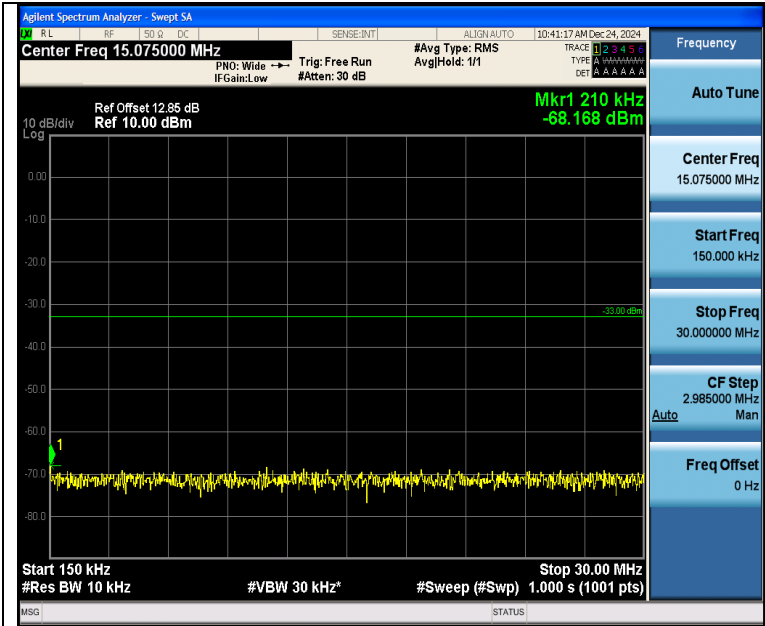
Band2_15MHz_QPSK_18675_1RB#74_0.15~30_0.15~30
