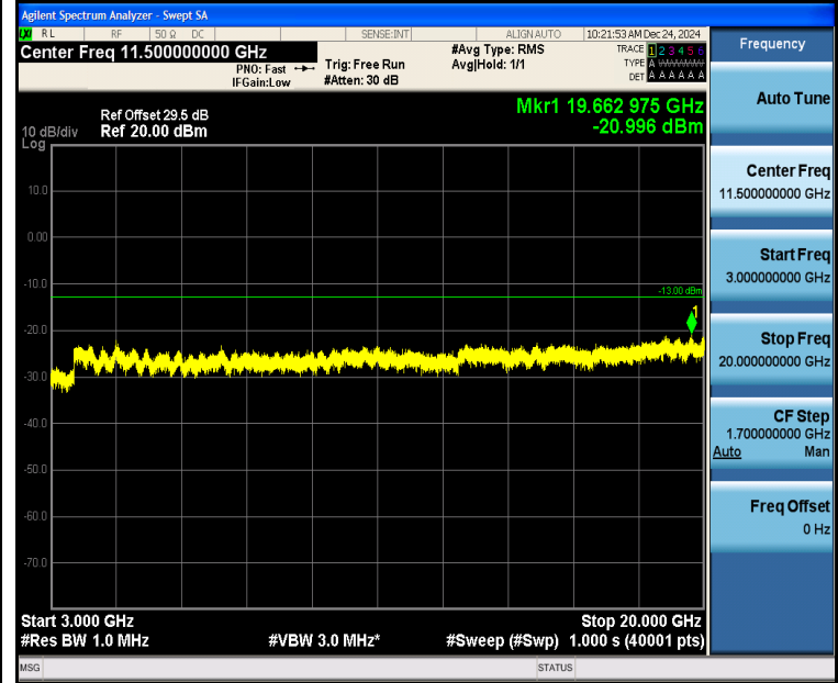
Band2_10MHz_16QAM_18650_1RB#0_3000~20000_3000~20000
