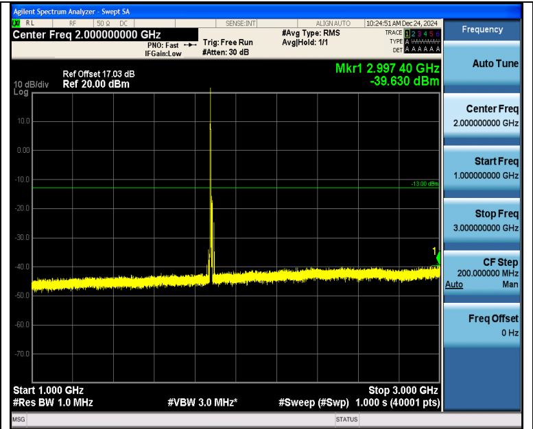
Band2_10MHz_QPSK_18900_1RB#0_1000~3000_1000~3000
