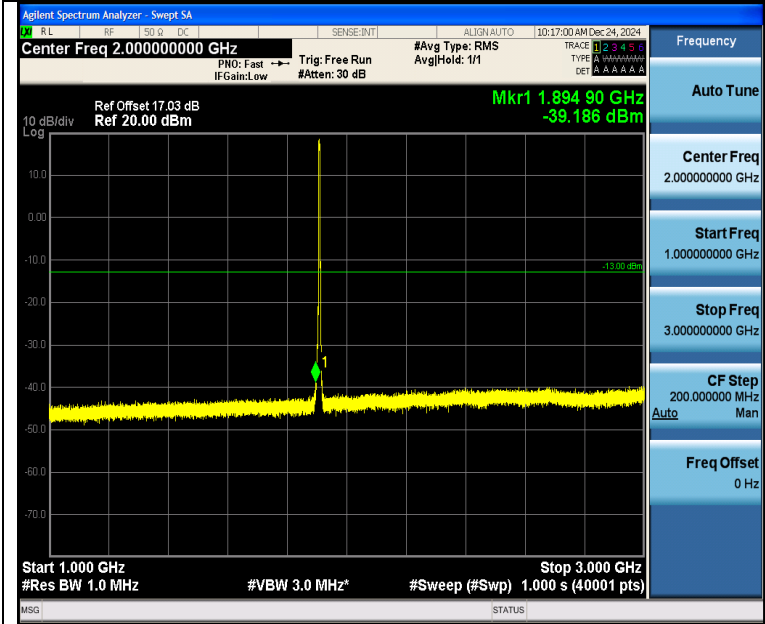
Band2_5MHz_16QAM_19175_25RB#0_1000~3000_1000~3000
