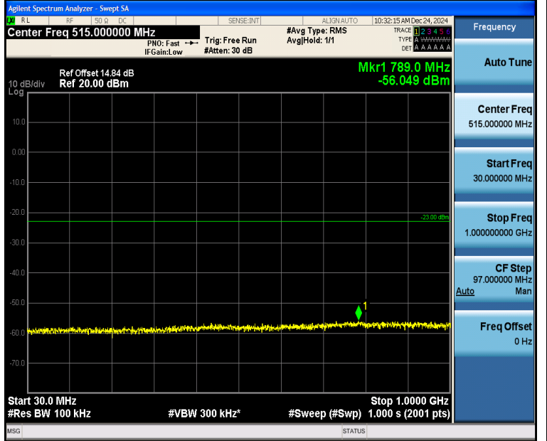
Band2_10MHz_16QAM_19150_1RB#49_30~1000_30~1000
