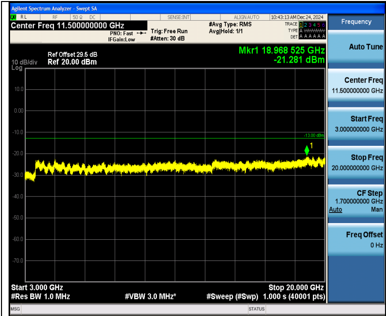
Band2_15MHz_16QAM_18675_1RB#74_3000~20000_3000~20000
