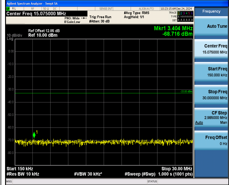
Band2_10MHz_16QAM_18650_1RB#49_0.15~30_0.15~30
