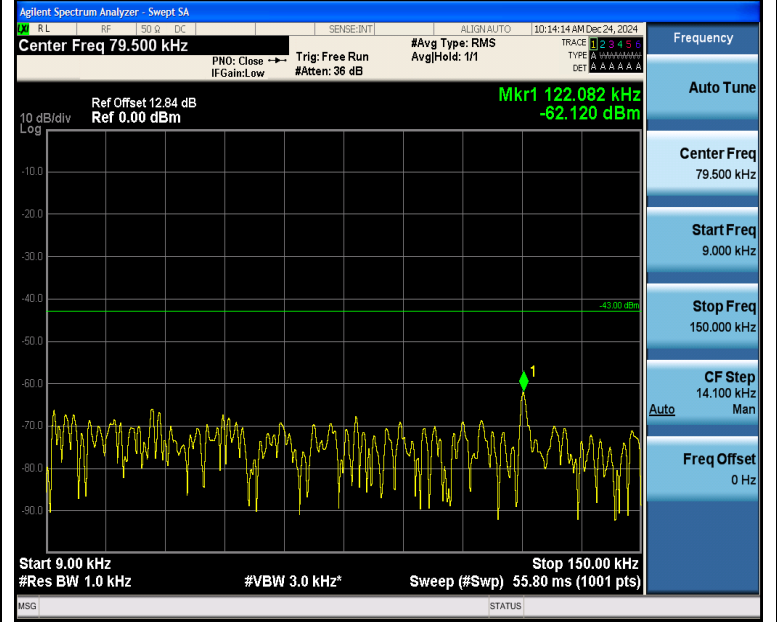
Band2_5MHz_16QAM_19175_1RB#24_0.009~0.15_0.009~0.15
