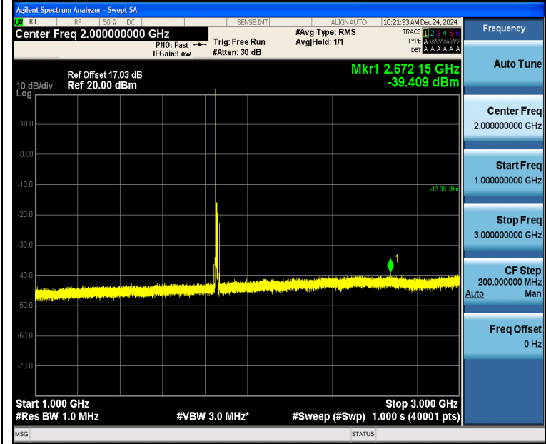
Band2_10MHz_16QAM_18650_1RB#0_1000~3000_1000~3000
