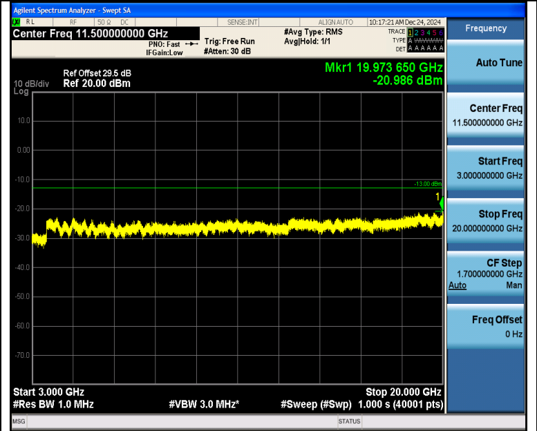
Band2_5MHz_16QAM_19175_25RB#0_3000~20000_3000~20000
