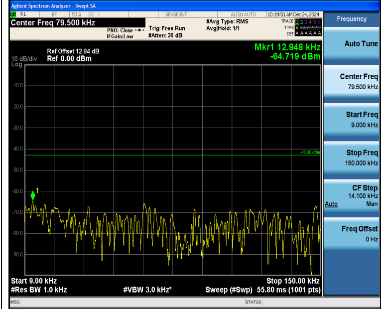
Band2_10MHz_QPSK_18650_1RB#0_0.009~0.15_0.009~0.15
