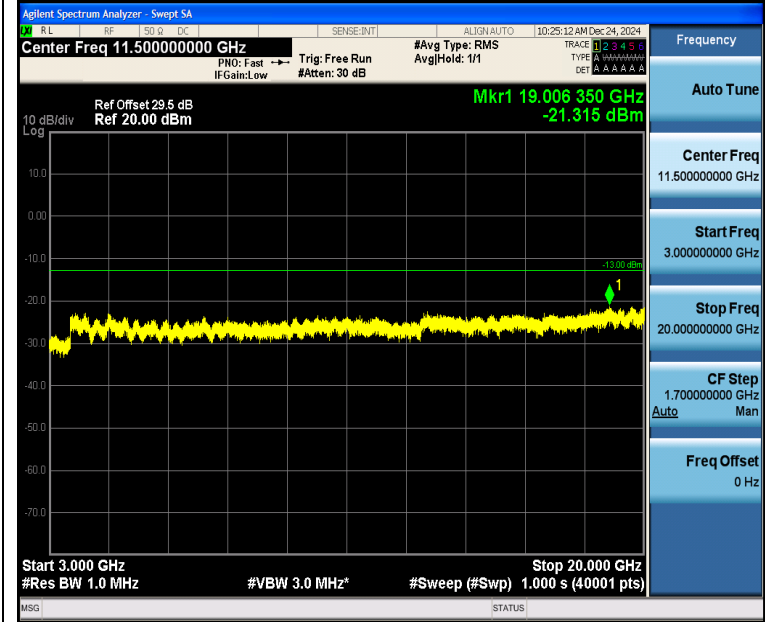
Band2_10MHz_QPSK_18900_1RB#0_3000~20000_3000~20000
