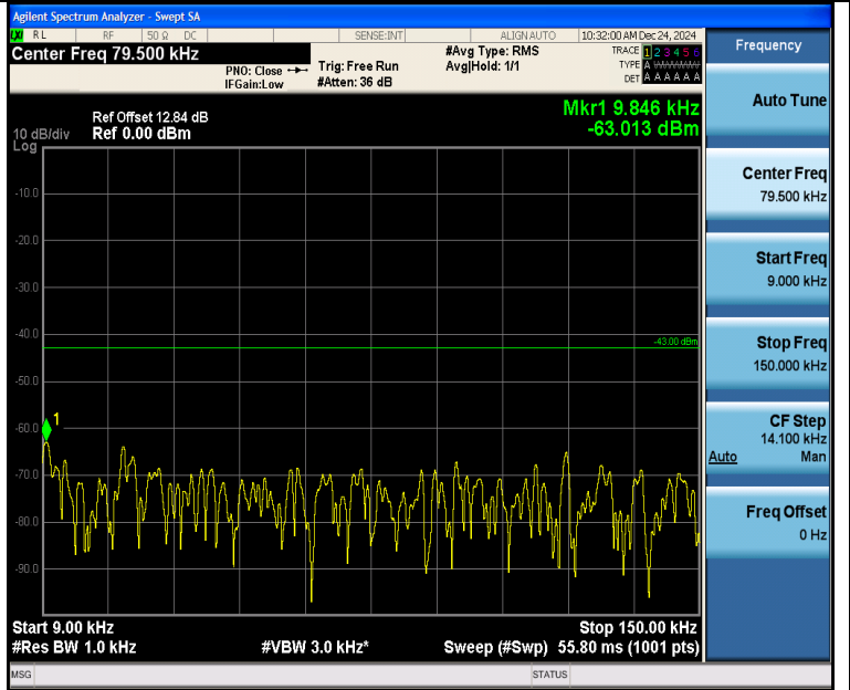
Band2_10MHz_16QAM_19150_1RB#49_0.009~0.15_0.009~0.15
