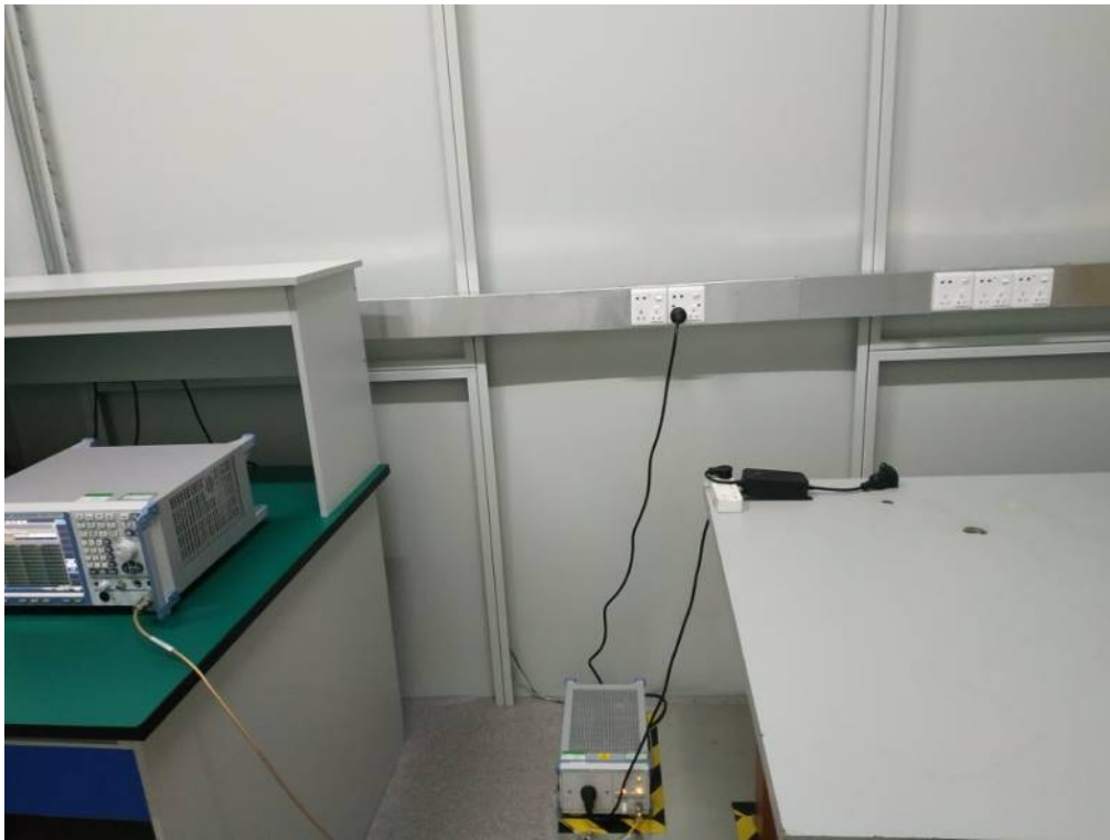
Radiated Emissions
