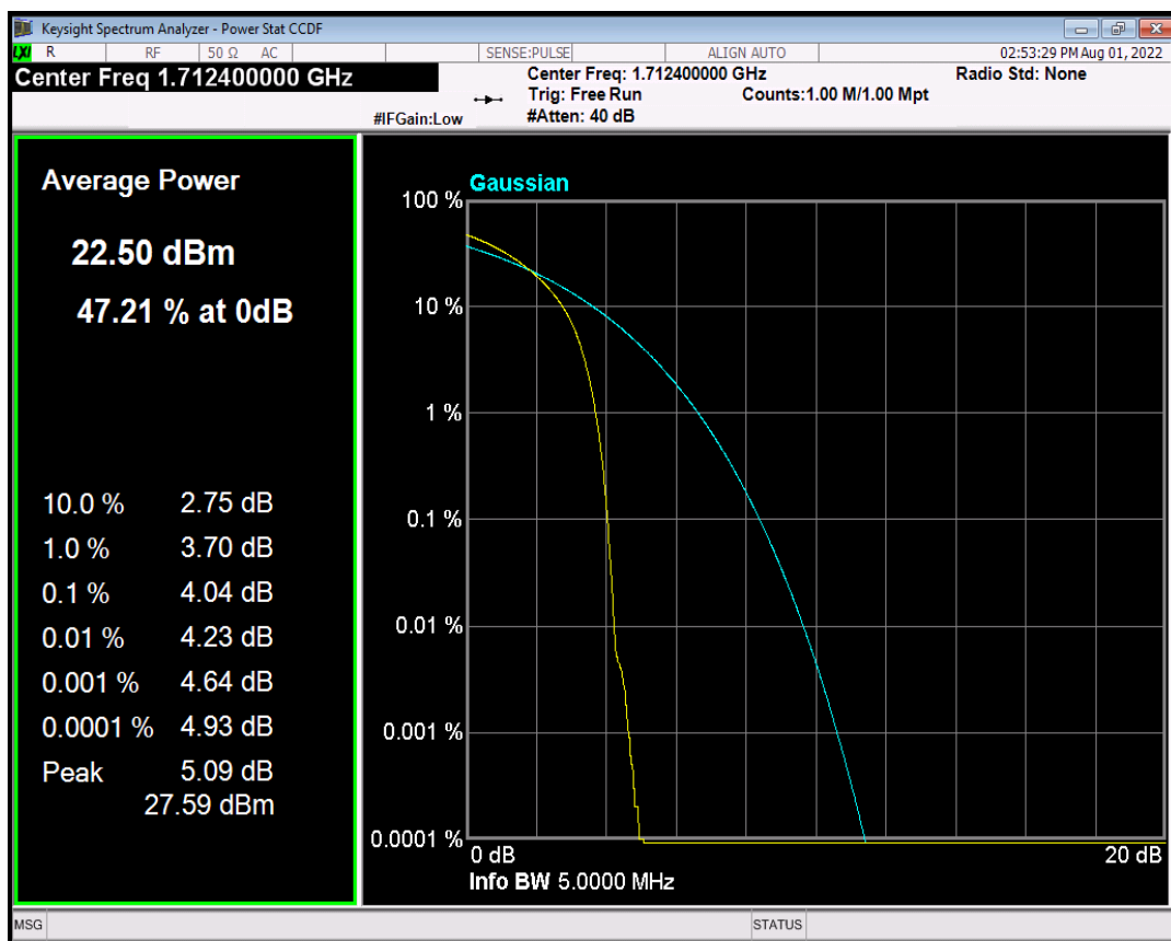
HSUPA Band4 Subtest4 Channel=1312
