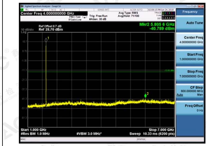
WCDMA 1700-HCH
