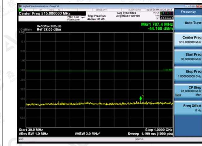
WCDMA 1700-HCH
