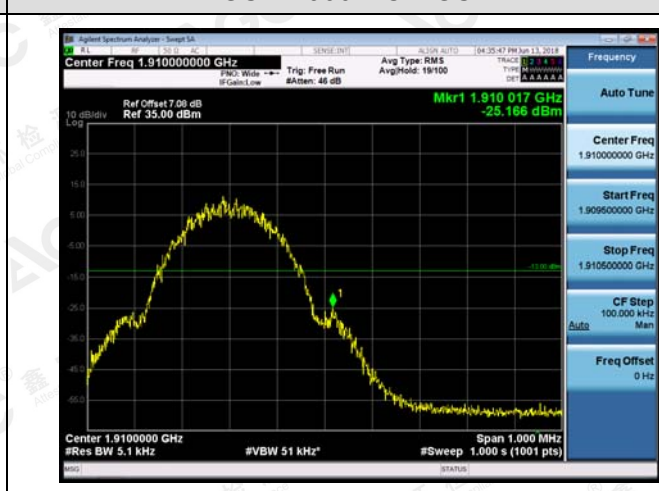
GSM 1900-HCH-GSM
