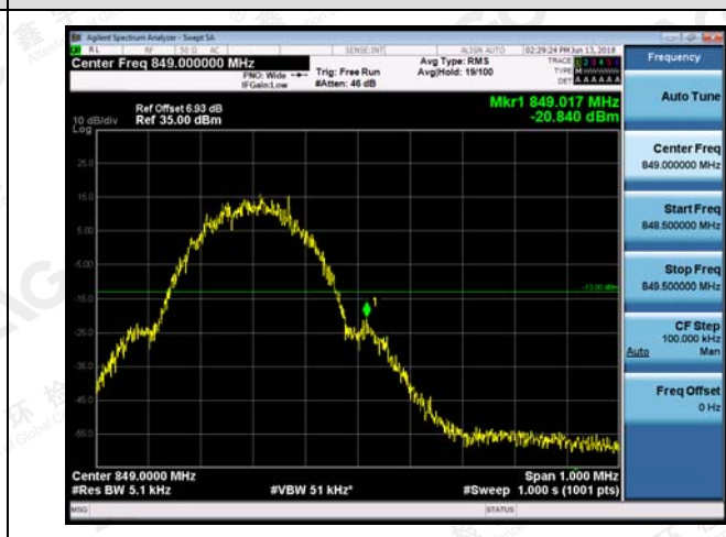
GSM 850-HCH-GSM
