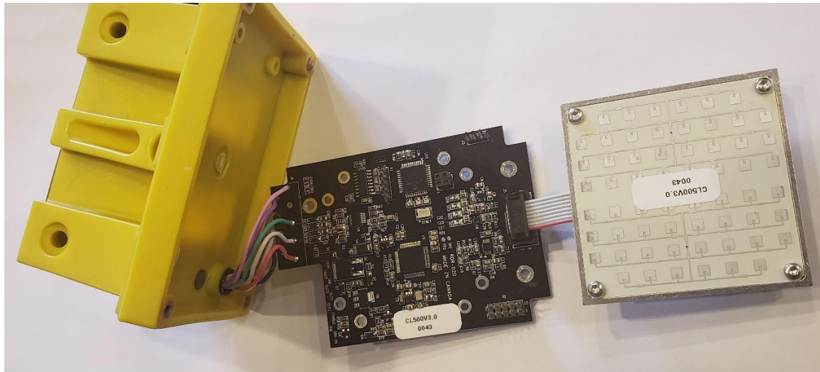
Internal photo: Housing PCB assembly, Transceiver
