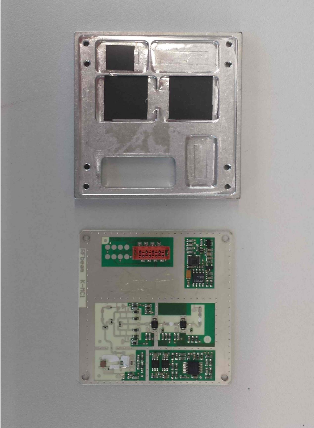
Internal_pcb&case
