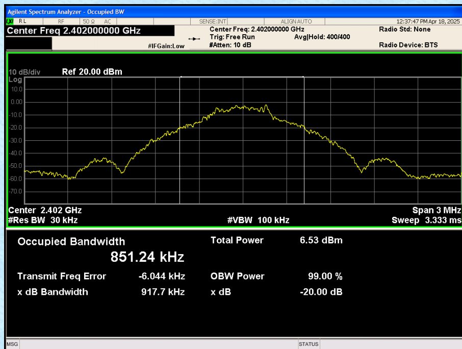
CH00: 2402MHz
