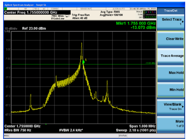
NB-IOT Band 4 QPSK 15KHz 1@0 CH-High
