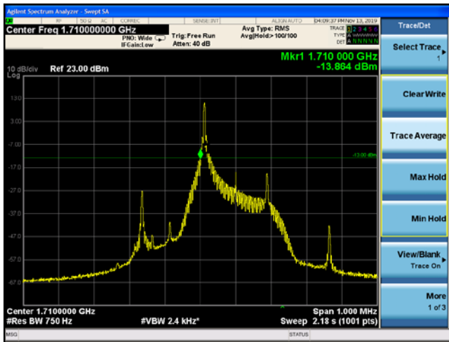
NB-IOT Band 4 QPSK 15KHz 1@0 CH-Low
