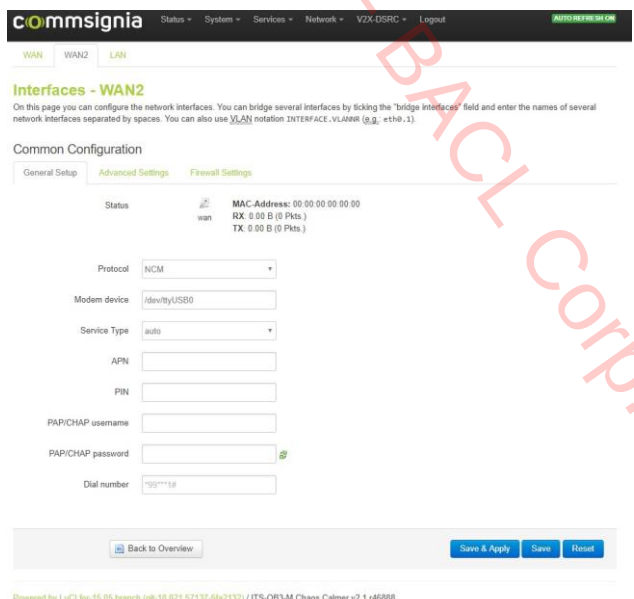
Figure 40: General settings for the cellular connection
