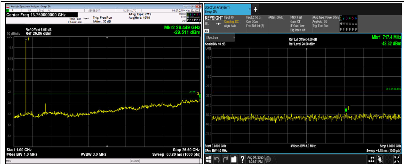
Band41-20MHz-64QAM-39750-1RB#0-Range2:100 0~27000MHz
