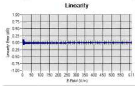
Linearity: +/-1.97% (+/-0.09dB)
