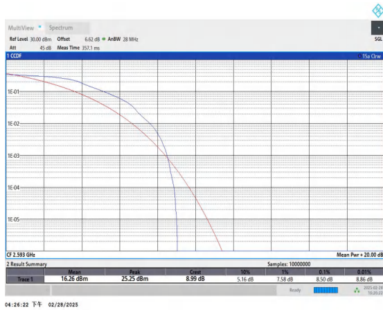
Band41-20MHz-QPSK-40620-1RB#0-PASS
