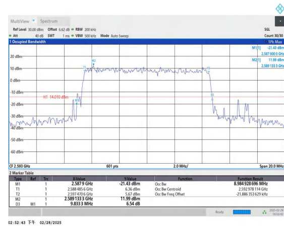
Band41-10MHz-QPSK-40620-50RB#0-PASS
