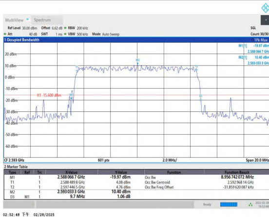
Band41-10MHz-16QAM-40620-50RB#0-PASS
