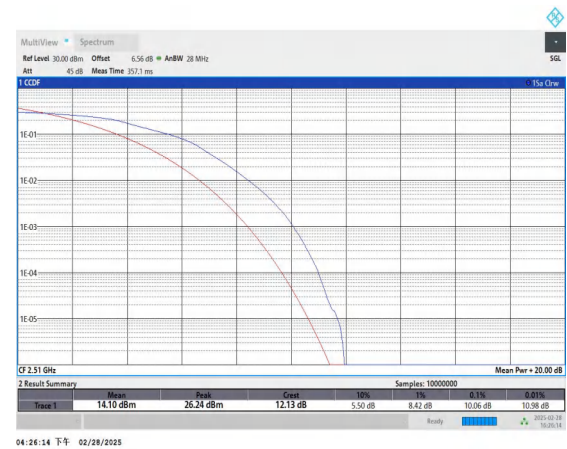
Band41-20MHz-16QAM-39790-100RB#0-PASS
