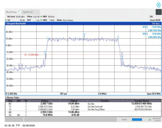
Band41-15MHz-QPSK-40620-75RB#0-PASS
