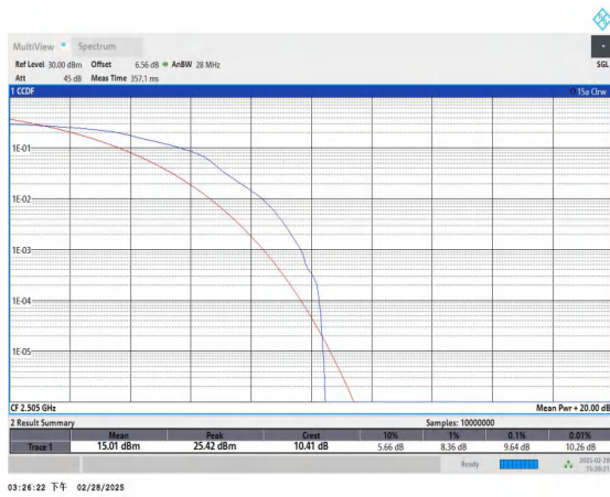
Band41-10MHz-16QAM-39740-1RB#0-PASS
