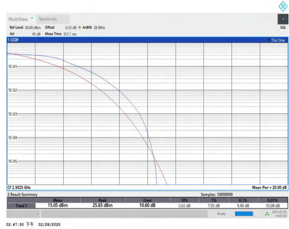
Band41-5MHz-QPSK-39715-25RB#0-PASS
