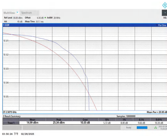
Band41-15MHz-16QAM-39765-1RB#0-PASS
