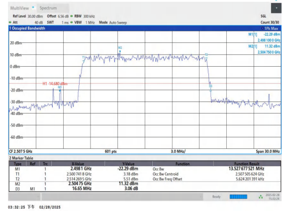
Band41-15MHz-16QAM-39765-75RB#0-PASS
