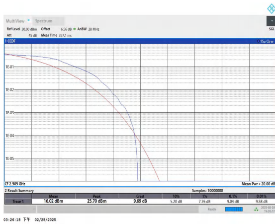
Band41-10MHz-QPSK-39740-1RB#0-PASS
