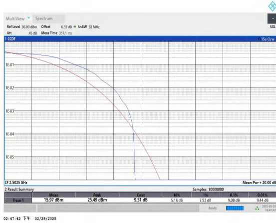
Band41-5MHz-QPSK-39715-1RB#0-PASS
