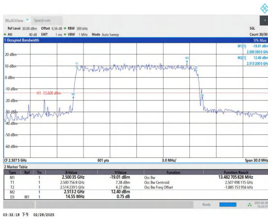
Band41-15MHz-QPSK-39765-75RB#0-PASS
