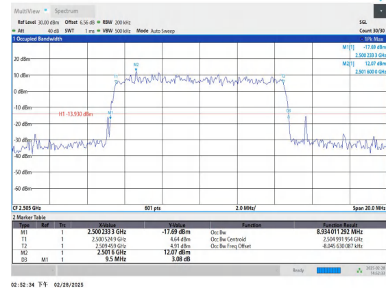
Band41-10MHz-16QAM-39740-50RB#0-PASS
