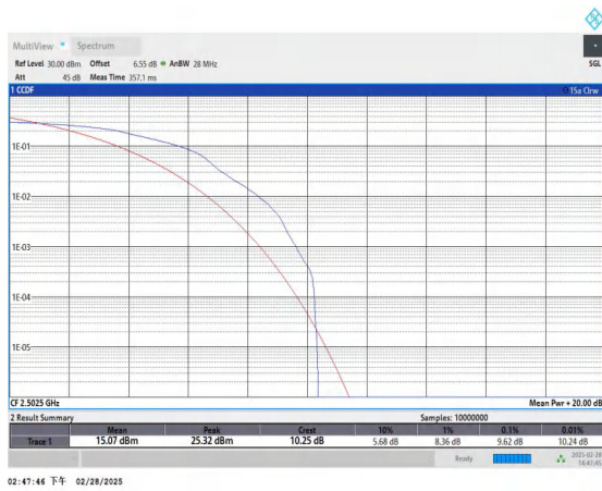
Band41-5MHz-16QAM-39715-1RB#0-PASS
