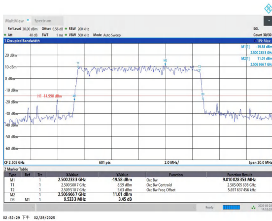
Band41-10MHz-QPSK-39740-50RB#0-PASS
