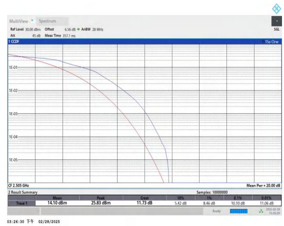
Band41-10MHz-16QAM-39740-50RB#0-PASS
