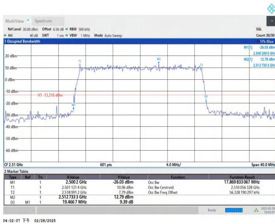
Band41-20MHz-QPSK-39790-100RB#0-PASS
