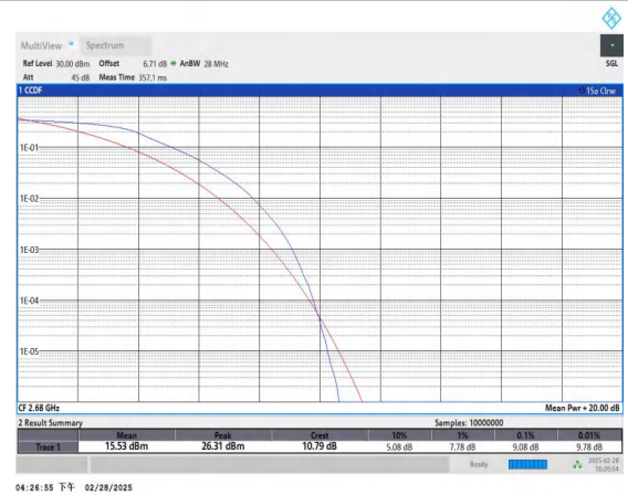
Band41-20MHz-QPSK-41490-100RB#0-PASS
