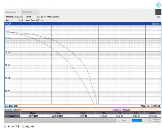
Band41-5MHz-16QAM-39715-25RB#0-PASS
