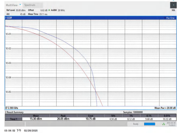
Band41-15MHz-QPSK-40620-75RB#0-PASS
