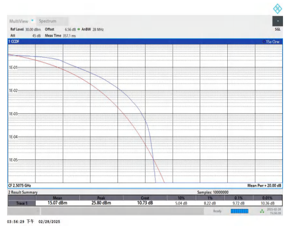
Band41-15MHz-QPSK-39765-75RB#0-PASS
