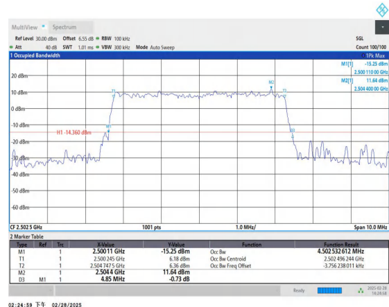
Band41-5MHz-16QAM-39715-25RB#0-PASS
