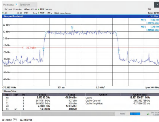
Band41-15MHz-QPSK-41515-75RB#0-PASS
