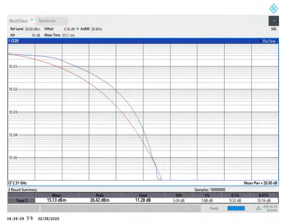
Band41-20MHz-QPSK-39790-100RB#0-PASS
