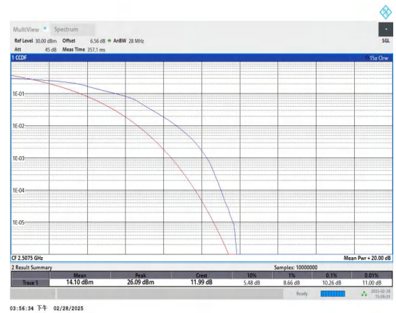
Band41-15MHz-16QAM-39765-75RB#0-PASS
