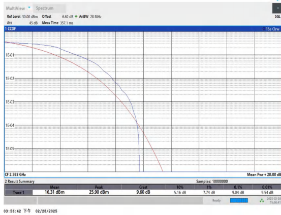
Band41-15MHz-QPSK-40620-1RB#0-PASS
