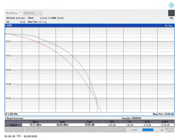
Band41-10MHz-QPSK-39740-50RB#0-PASS
