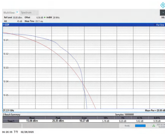
Band41-20MHz-16QAM-39790-1RB#0-PASS
