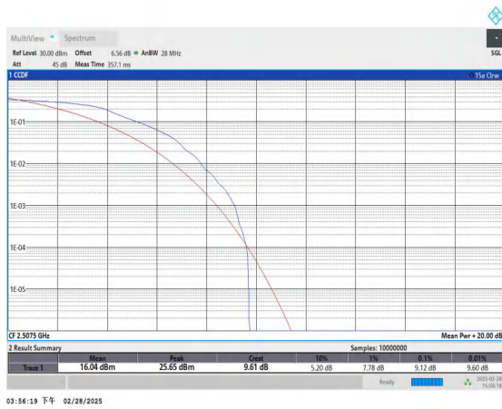
Band41-15MHz-QPSK-39765-1RB#0-PASS
