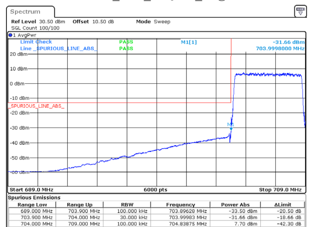
5MHz_Low_16QAM_25@0
