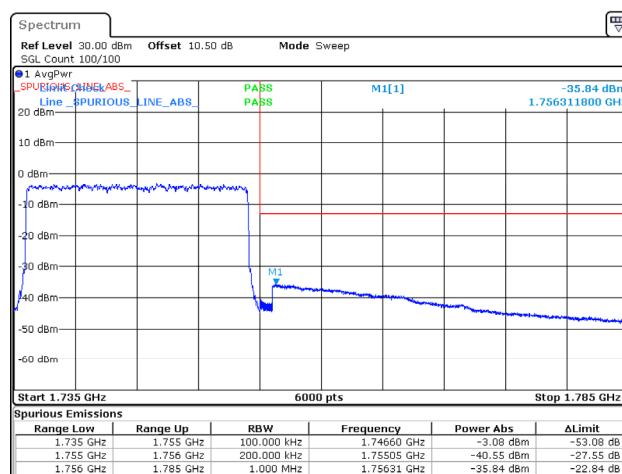
20MHz_High_16QAM_100@0
