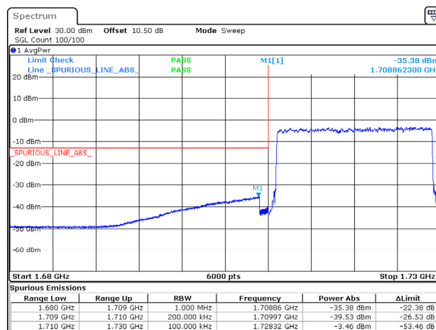
20MHz_Low_16QAM_100@0
