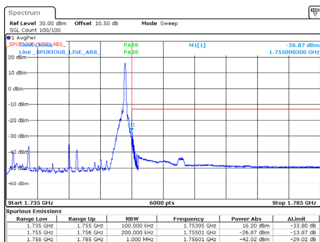
20MHz_High_16QAM_1@99
