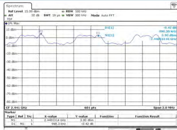
8-DPSK
