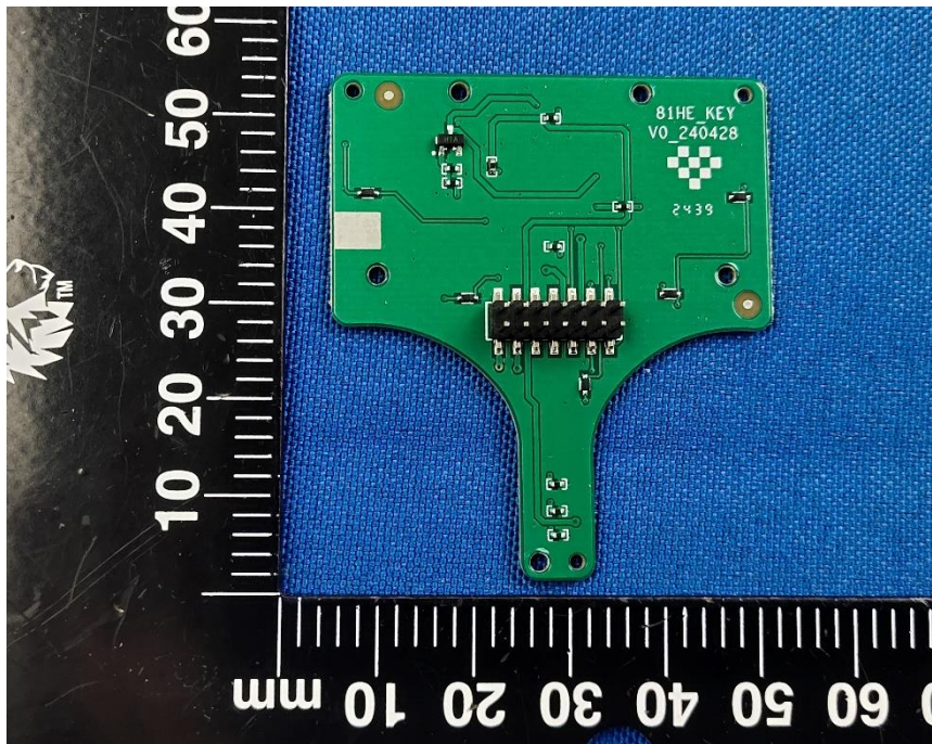
SECONDARY BOARD 1 TOP VIEW
