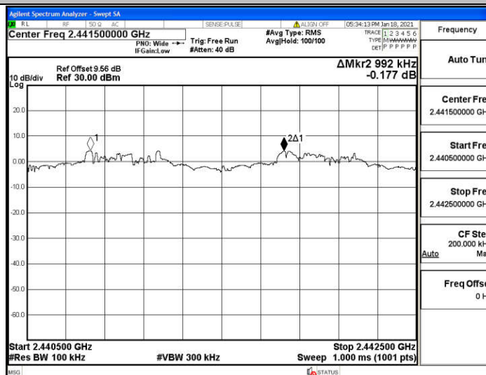
3DH5_Ant3_Hop
