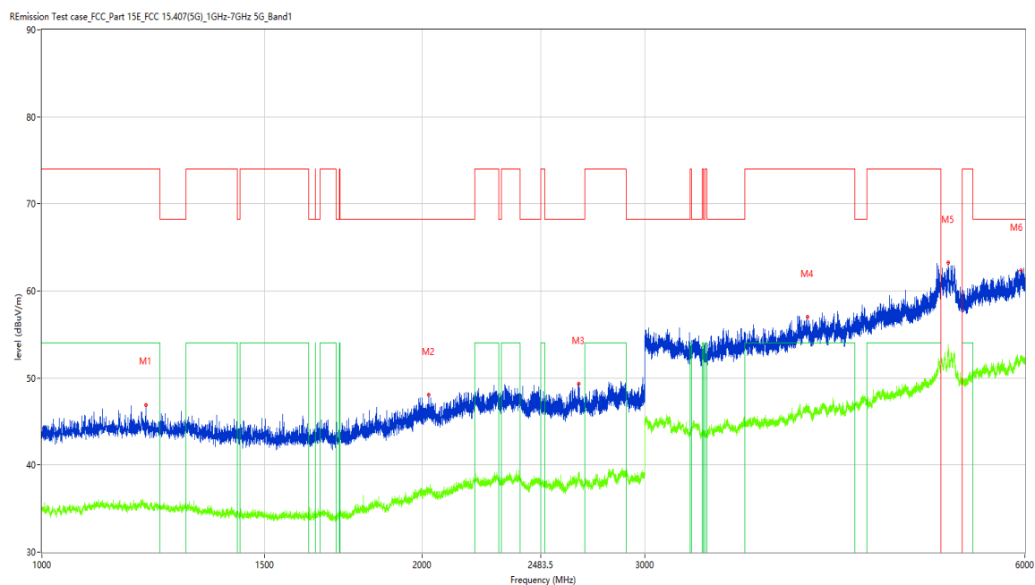
Figure 104: Spurious Emission, 1GHz – 10 th Harmonic, 802.11a, 5240MHz 1GHz-6GHz, Horizontal
