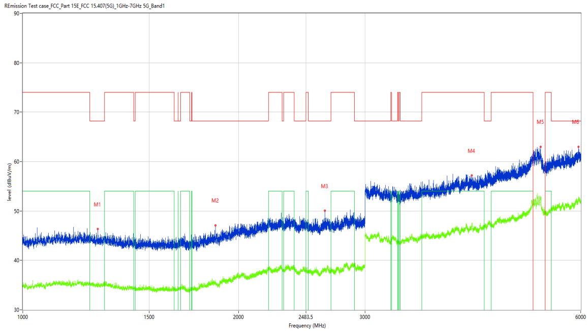
Figure 103: Spurious Emission, 1GHz – 10 th Harmonic, 802.11a, 5220MHz 1GHz-6GHz, Horizontal
