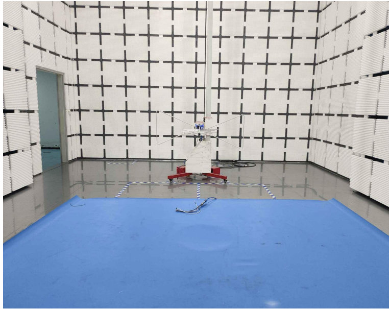
Radiated Emissions which fall in the restricted bands
