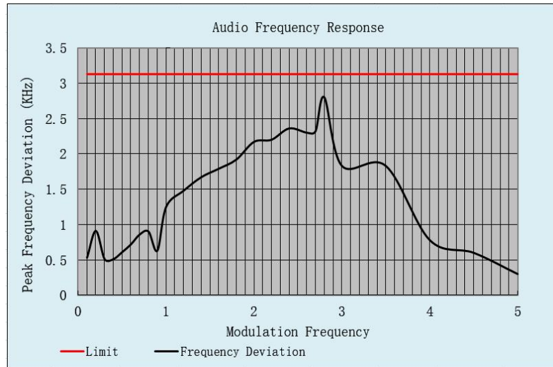
Channel 1: 462.5625MHz
