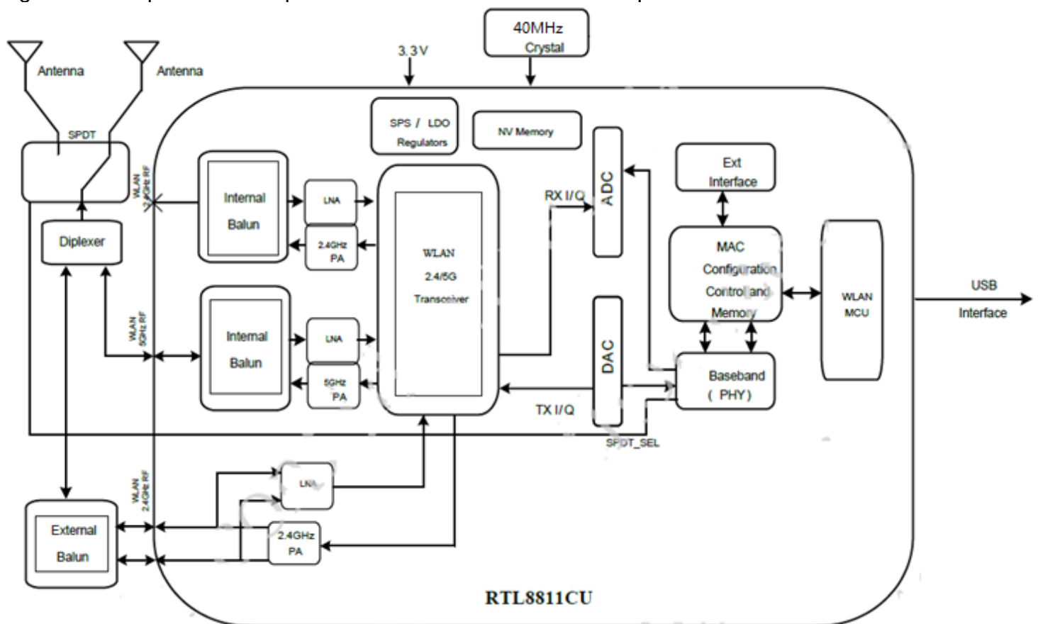
Figure 1 WF-R11C-UWD1 Block Diagram
