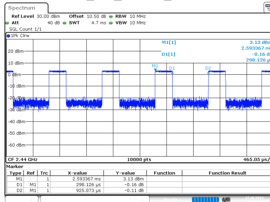
BLE_1M_Middle_Channel
