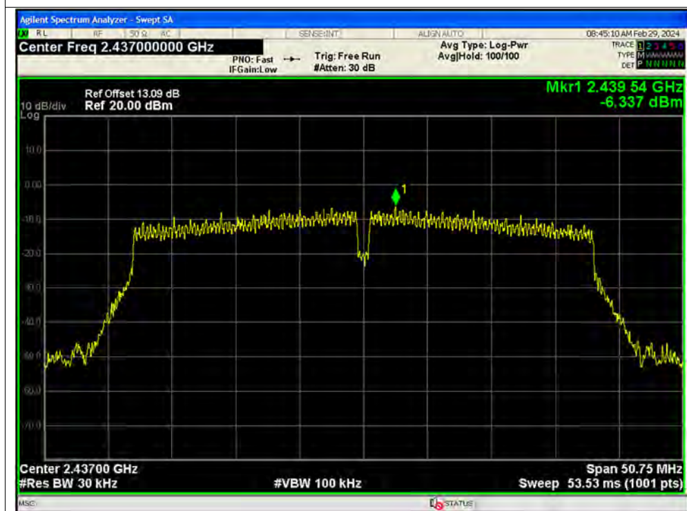
PSD NVNT n40 2437MHz Ant1 SISO
