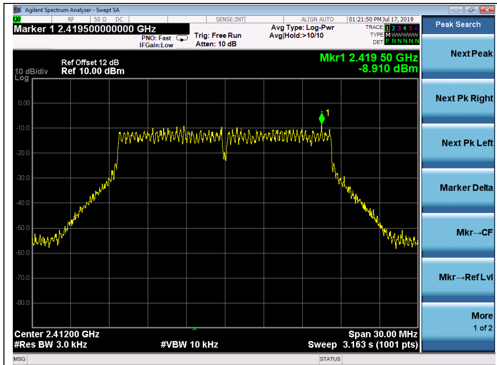
(Channel = 1, 802.11g)
