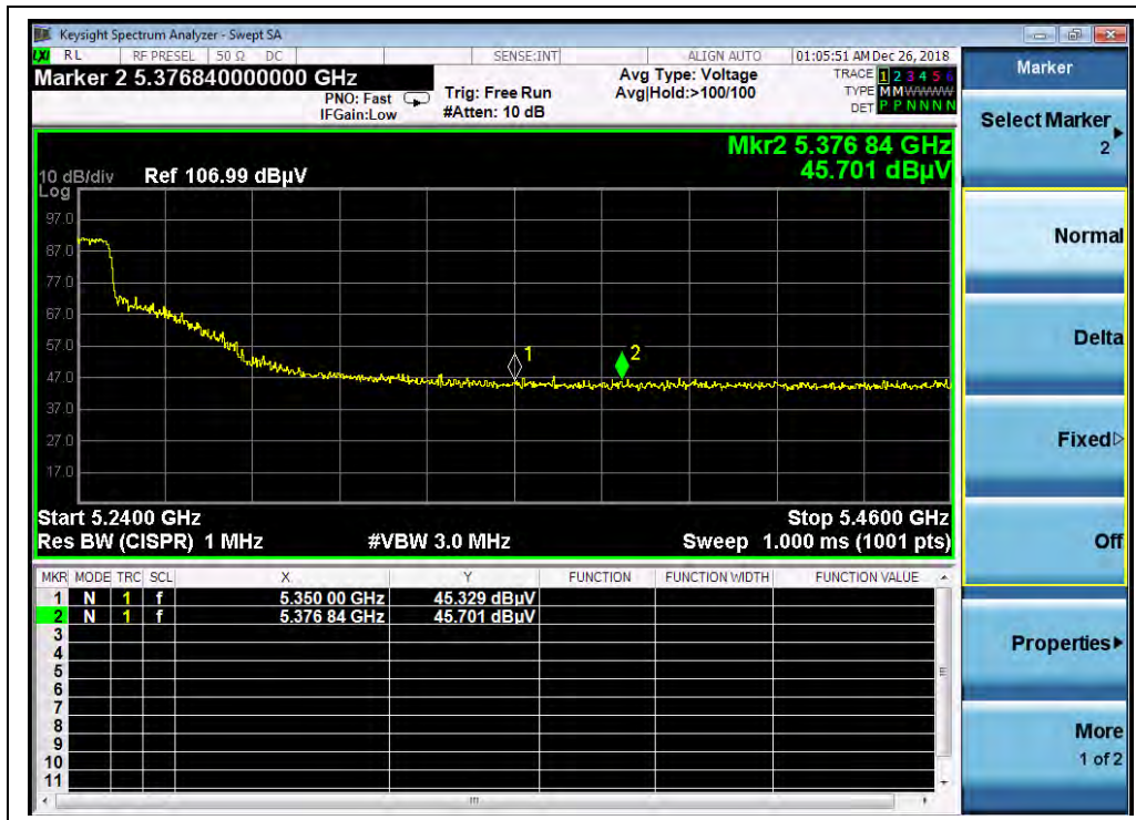
(Channel 46, PEAK, 802.11ac (VHT40))
