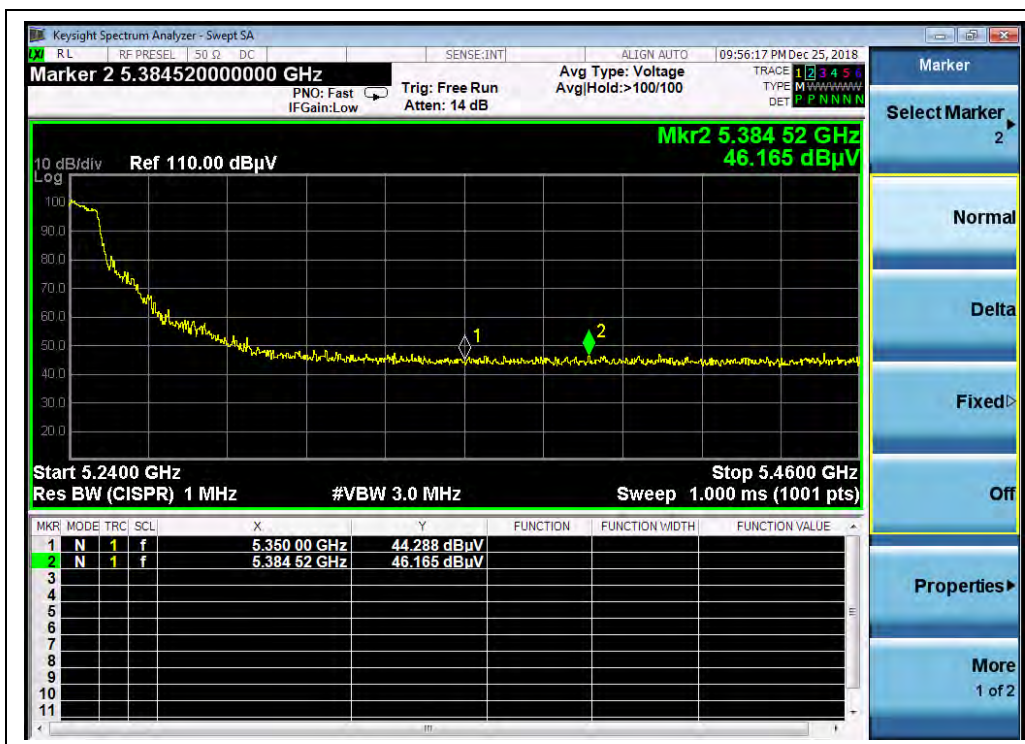
(Channel 48, PEAK, 802.11a)
