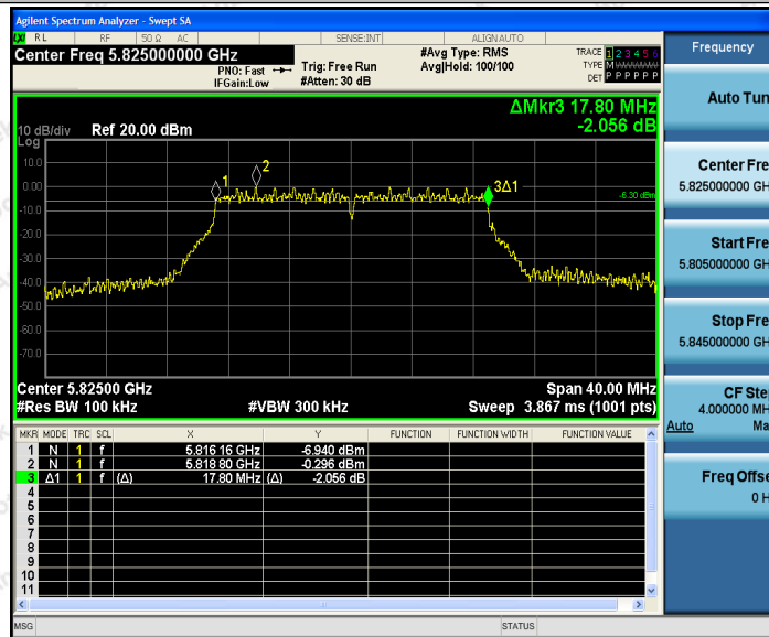
11AC20SISO_Ant2_5825
