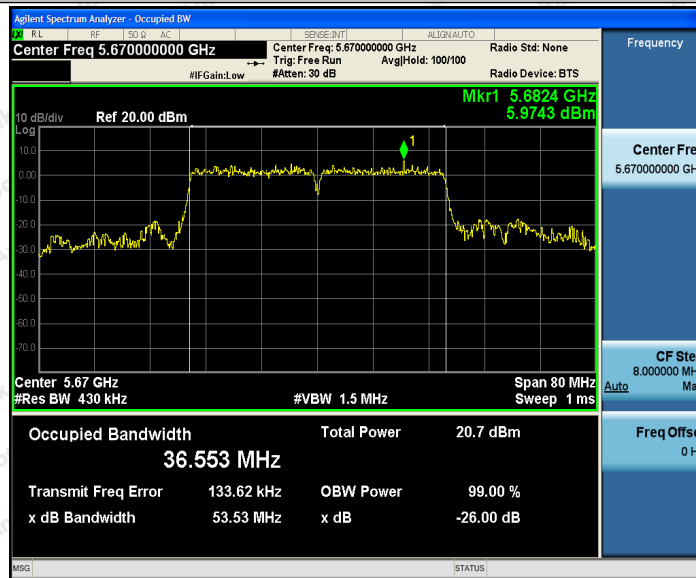
11N40SISO_Ant2_5670
