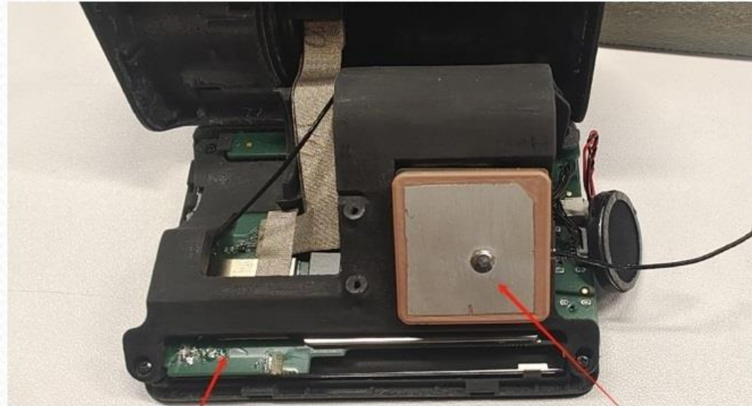
WiFi/BT Antenna
