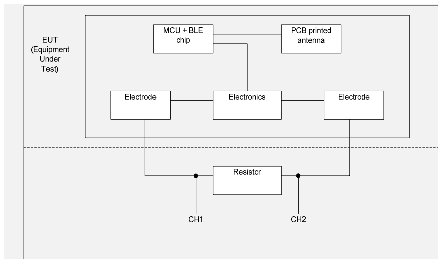
Figure 1. Nerivio Migra block diagram.
