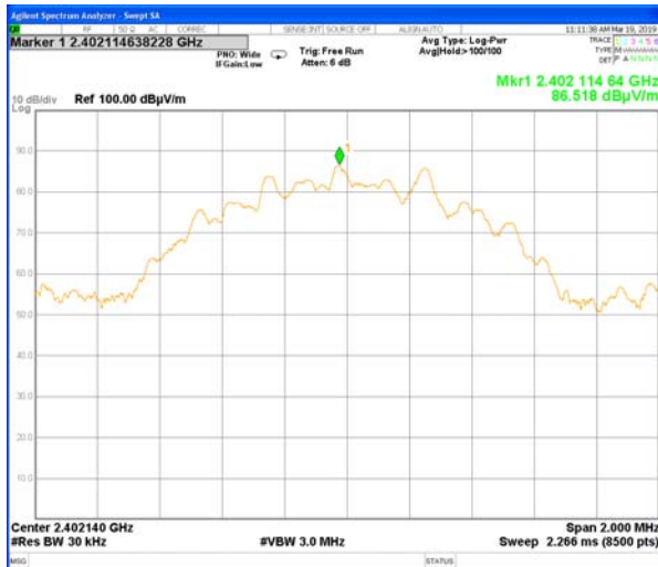
Plot # 7. Carrier frequency – 2402 MHz
