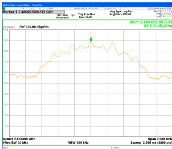
Plot # 9. Carrier frequency – 2480 MHz
