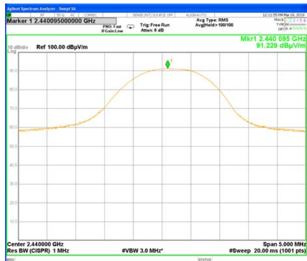
Plot # 5. Carrier frequency – 2440 MHz
