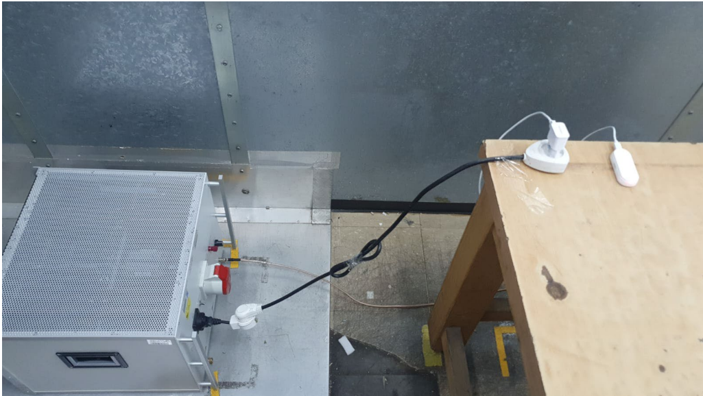
Conducted emission test set up
