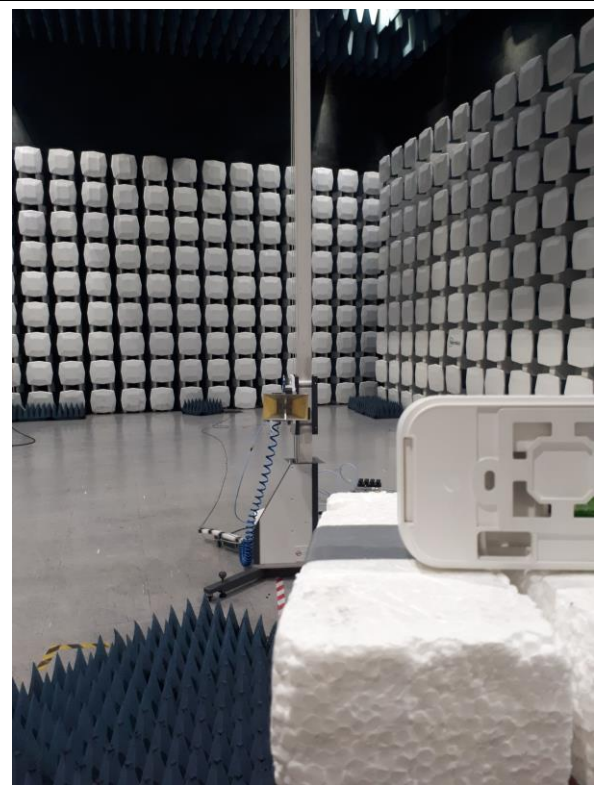
Radiated Emissions 1 – 2.5 GHz seen from device
