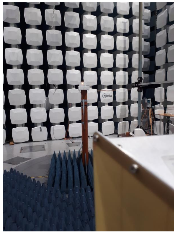
Radiated Emissions 1 – 2.5 GHz seen from antenna
