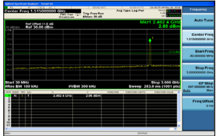
802.11g: Spurious Emission Test Data CH-High
