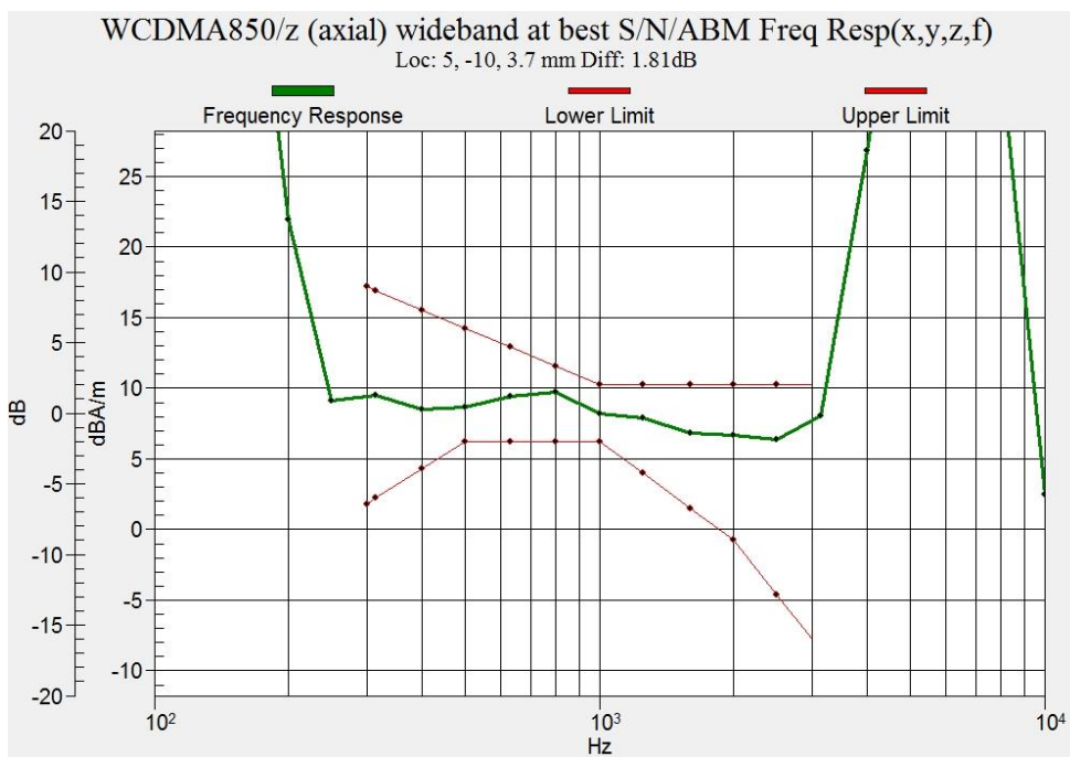
Figure B.3 Frequency Response of WCDMA B5
