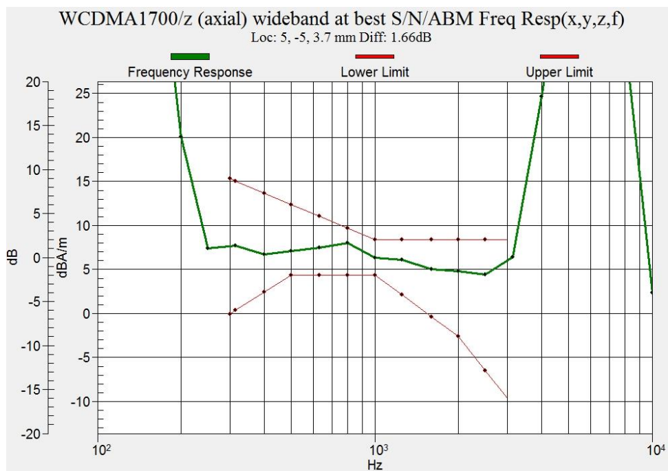
Figure B.2 Frequency Response of WCDMA B4
