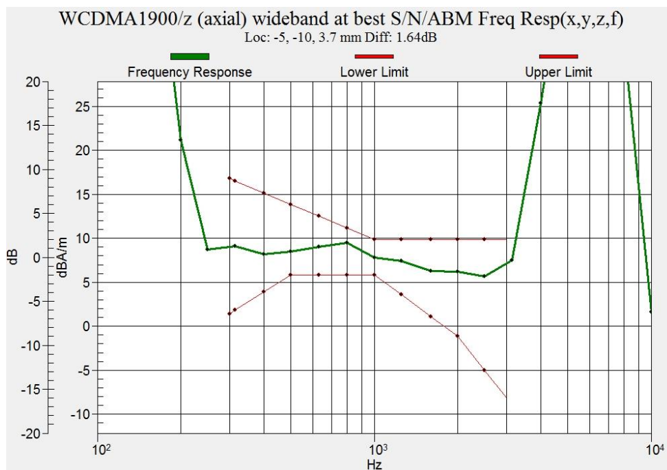
Figure B.1 Frequency Response of WCDMA B2
