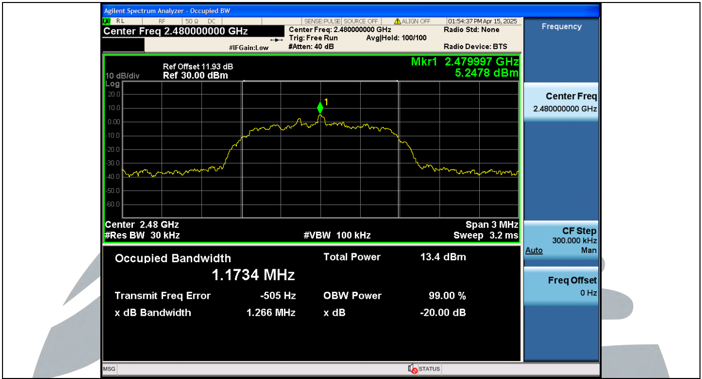
2DH5-Ant1-2480 MHz
