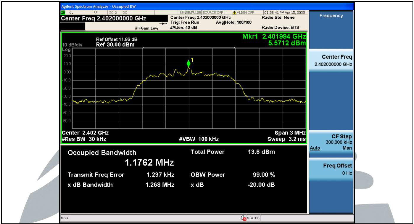
2DH5-Ant1-2402 MHz
