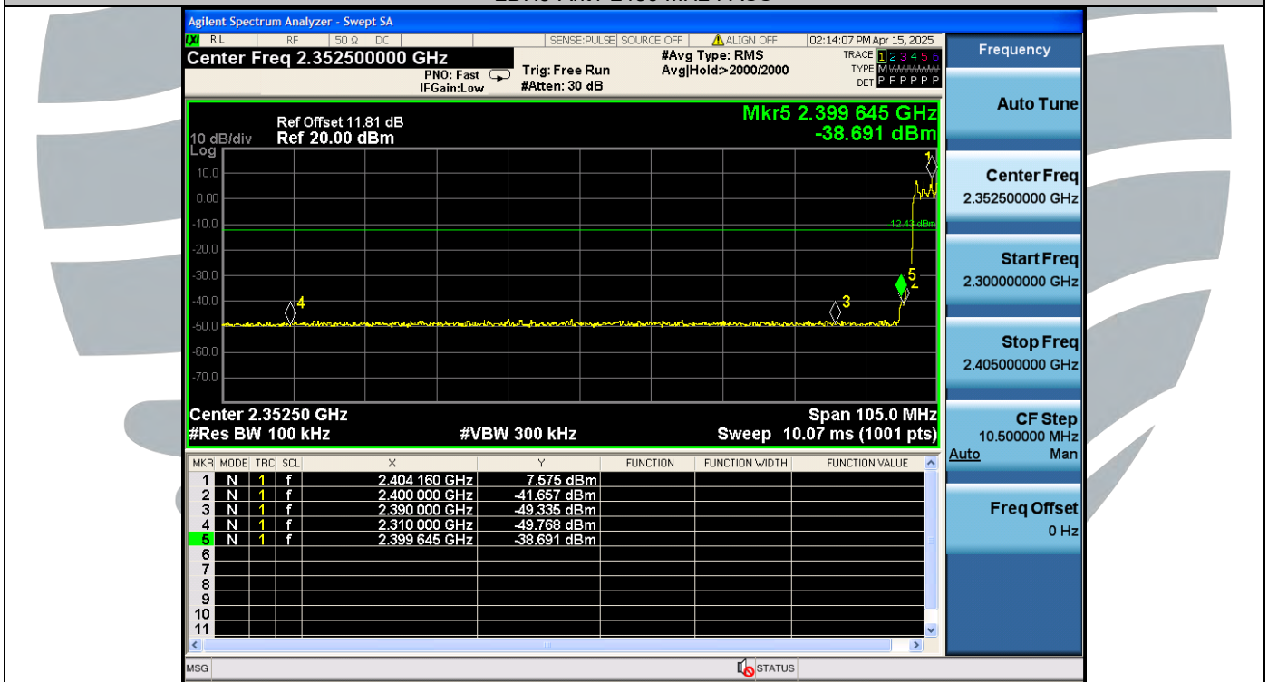
2DH5-Ant1-Hop_2402-PASS
