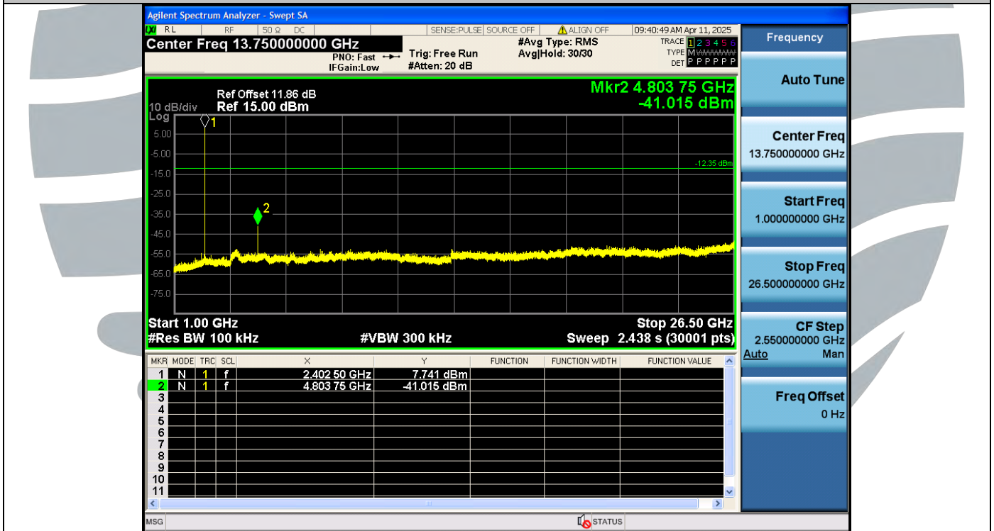
DH5-Ant1-2402 MHz-1000~26500 MHz-PASS
