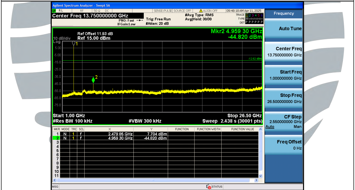
DH5-Ant1-2480 MHz-1000~26500 MHz-PASS
