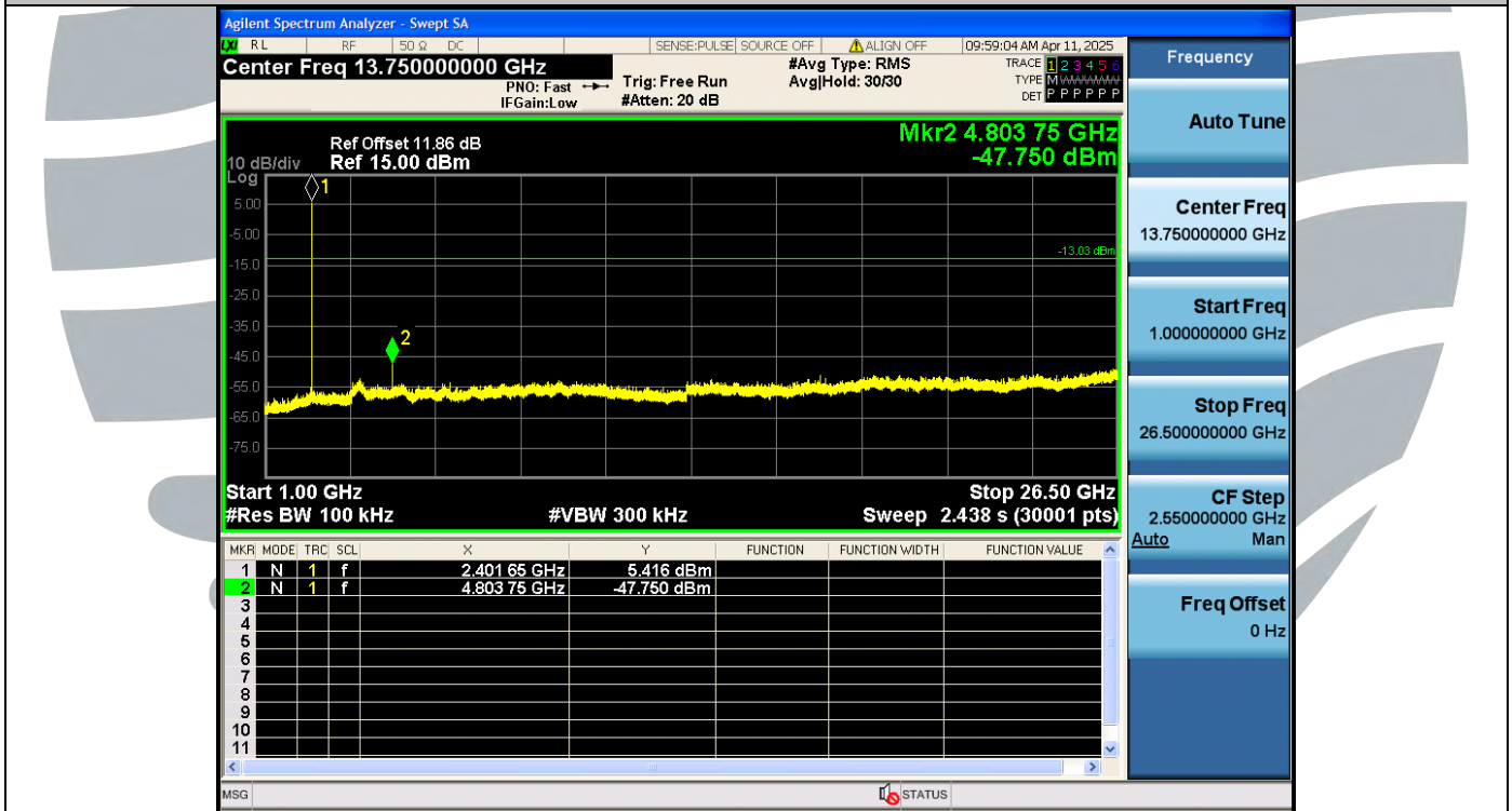
3DH5-Ant1-2402 MHz-1000~26500 MHz-PASS
