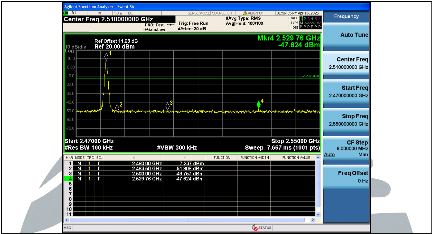
DH5-Ant1-2480 MHz-PASS
