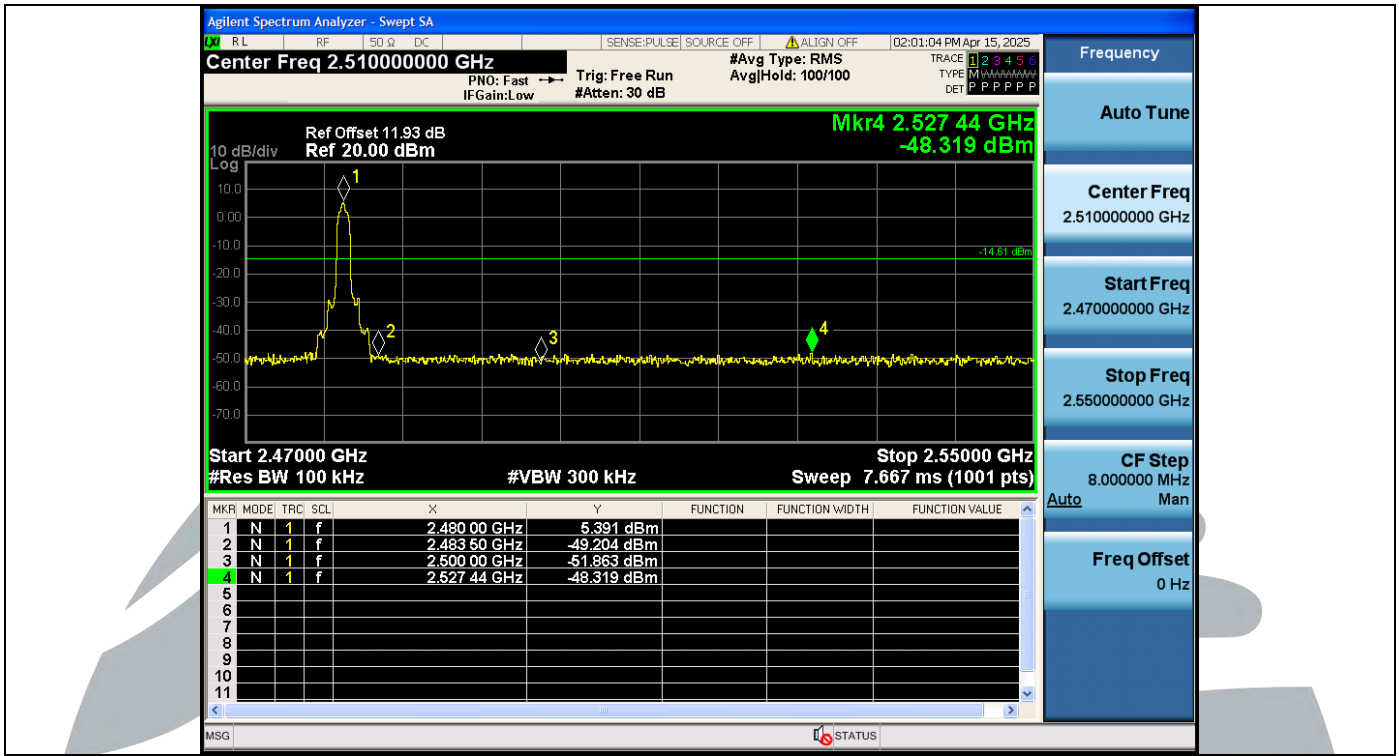
2DH5-Ant1-2480 MHz-PASS
