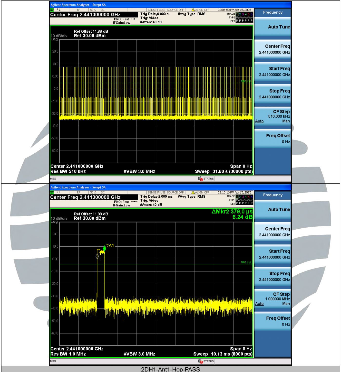
2DH1-Ant1-Hop-PASS
