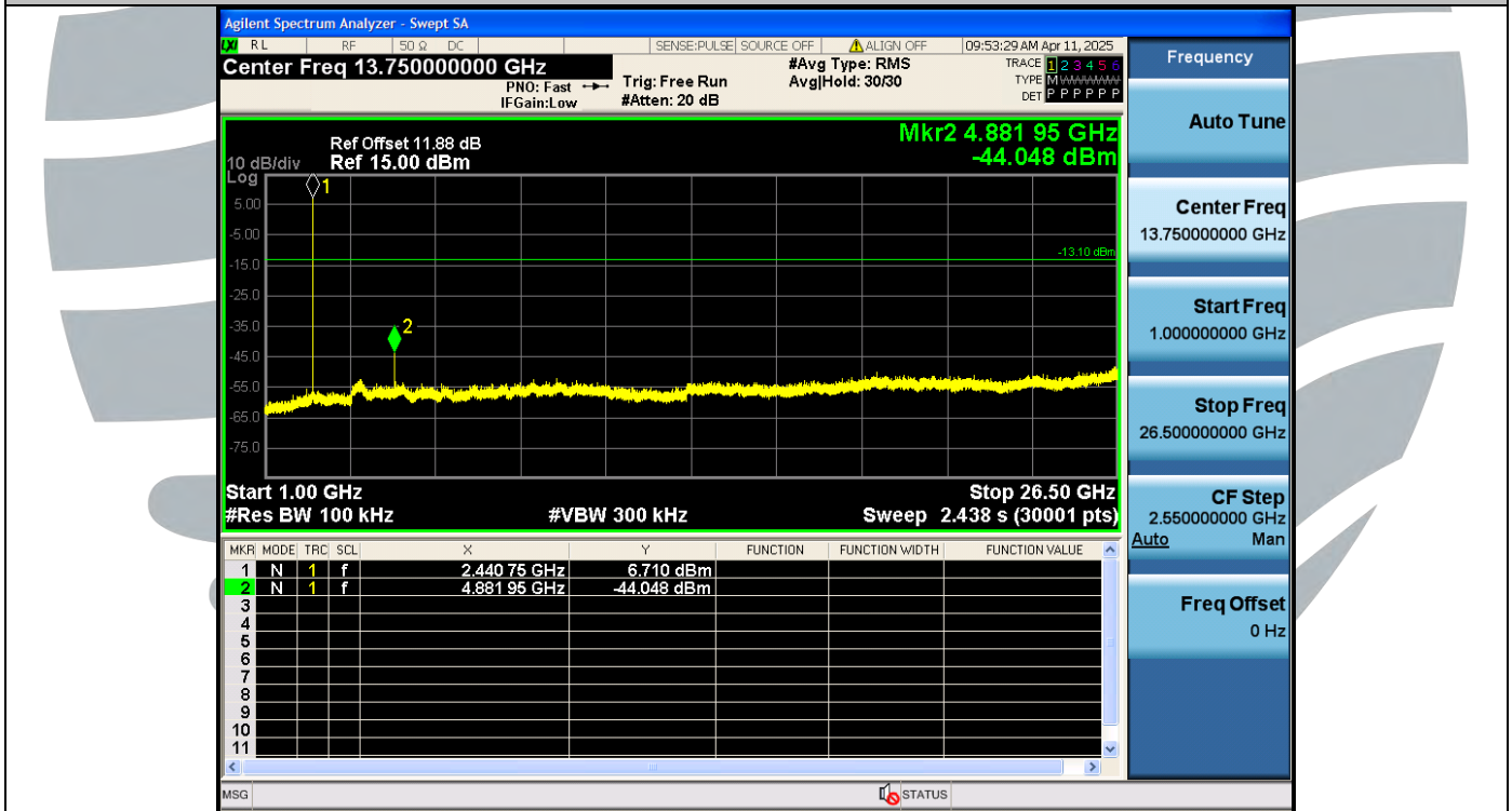
2DH5-Ant1-2441 MHz-1000~26500 MHz-PASS
