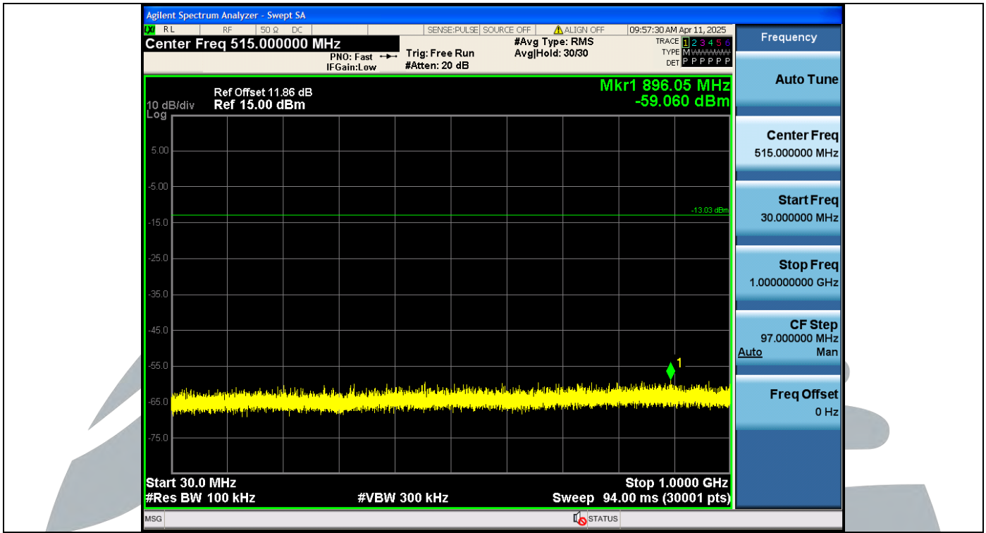
3DH5-Ant1-2402 MHz-30~1000 MHz-PASS
