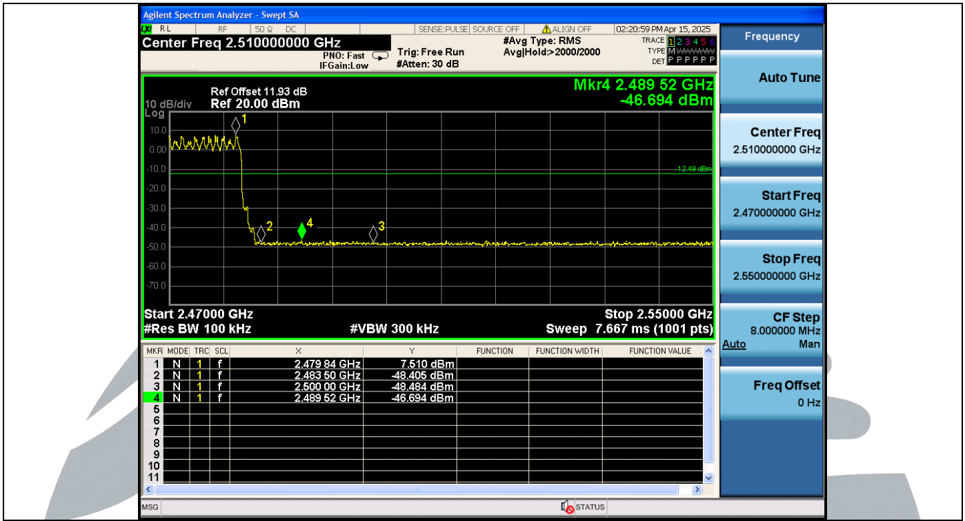
2DH5-Ant1-Hop_2480-PASS
