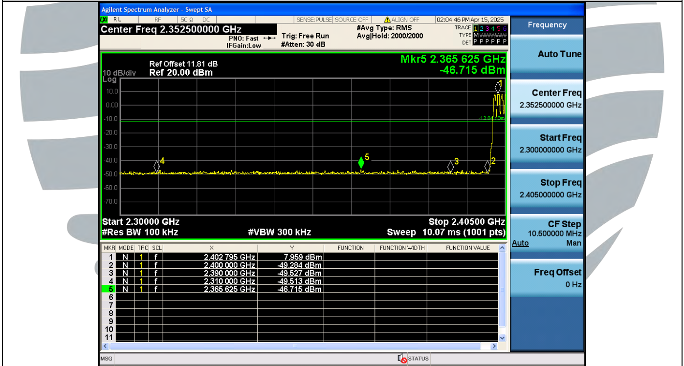
DH5-Ant1-Hop_2402-PASS
