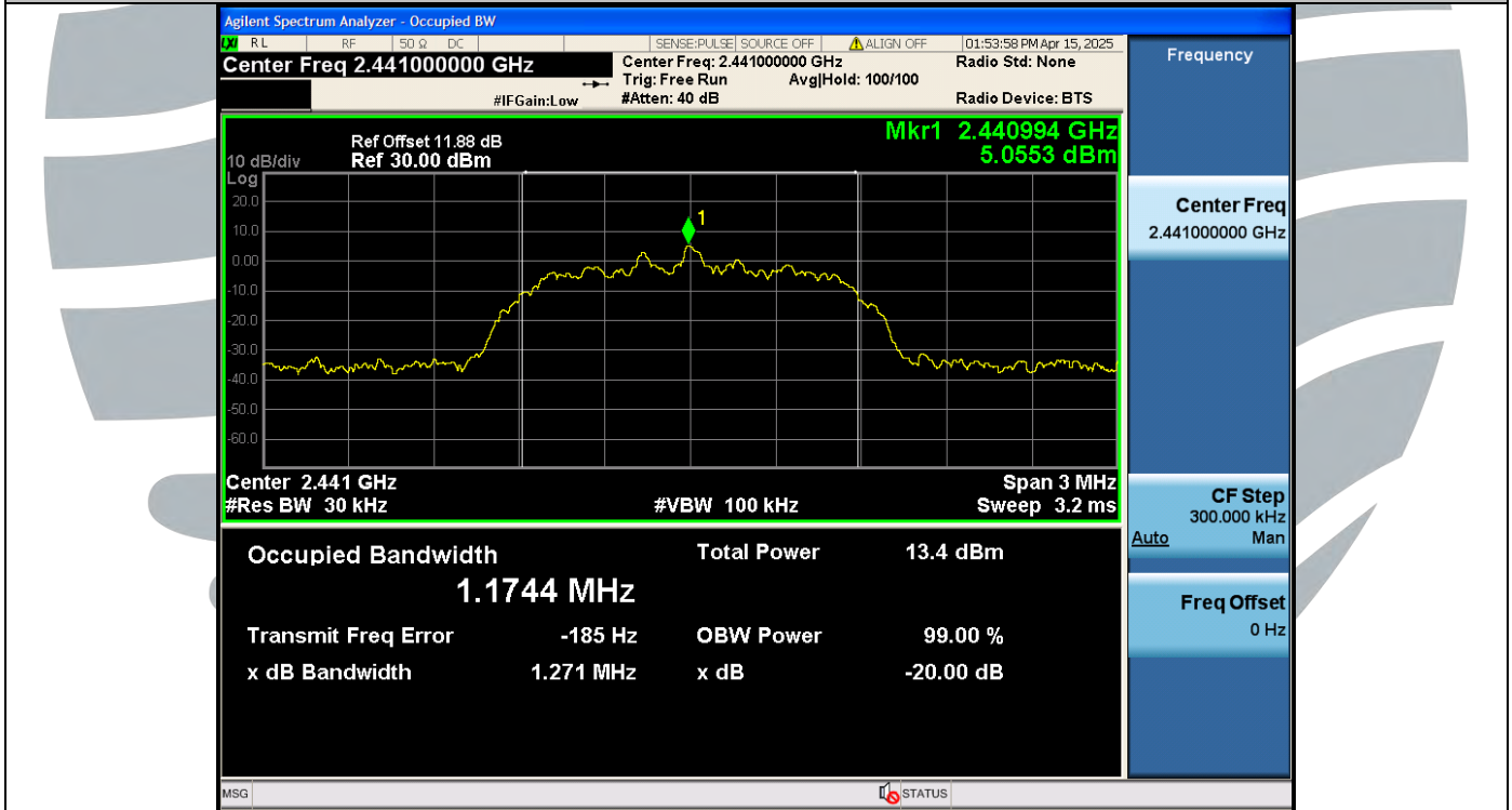
2DH5-Ant1-2441 MHz
