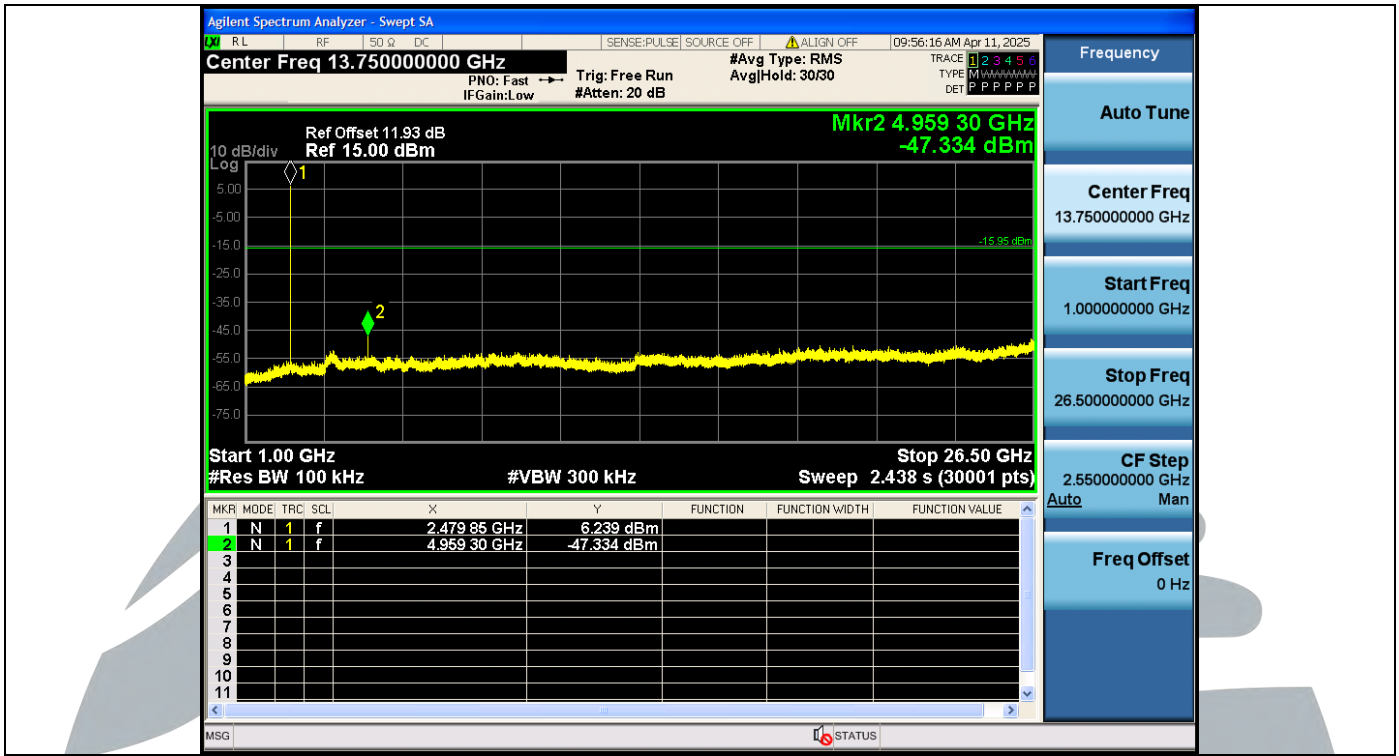
2DH5-Ant1-2480 MHz-1000~26500 MHz-PASS
