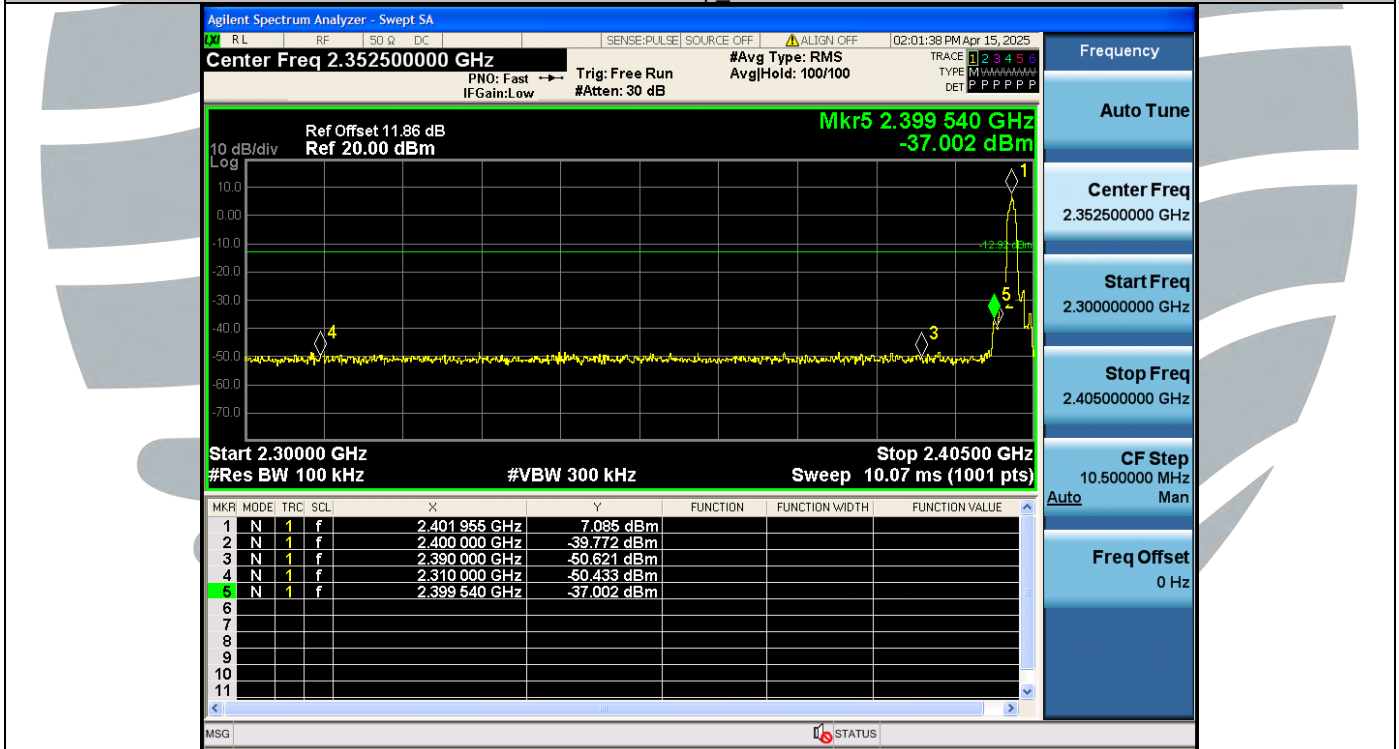
3DH5-Ant1-2402 MHz-PASS
