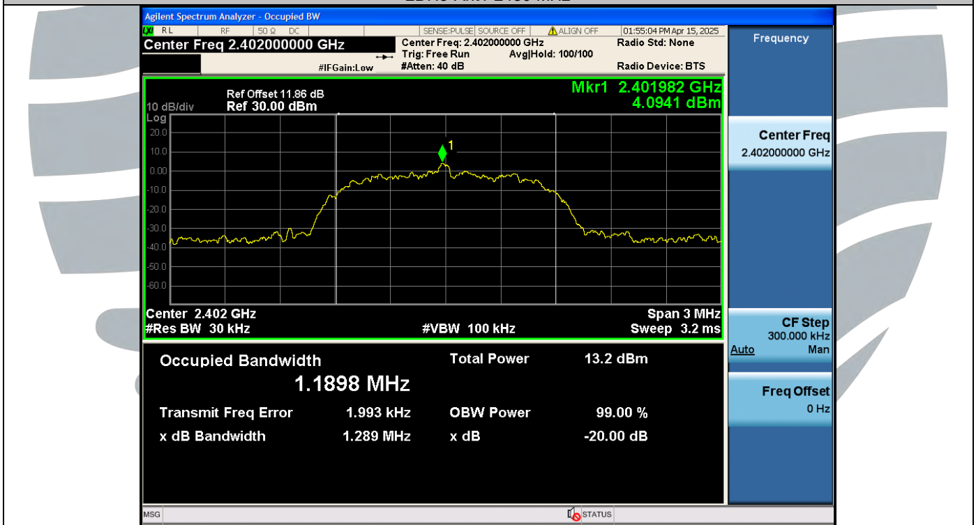
3DH5-Ant1-2402 MHz
