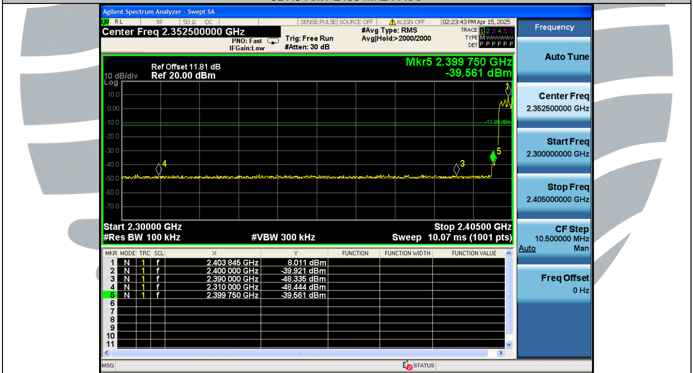
3DH5-Ant1-Hop_2402-PASS
