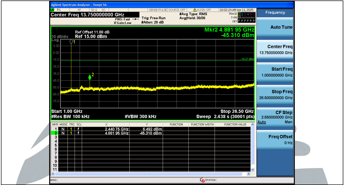
3DH5-Ant1-2441 MHz-1000~26500 MHz-PASS
