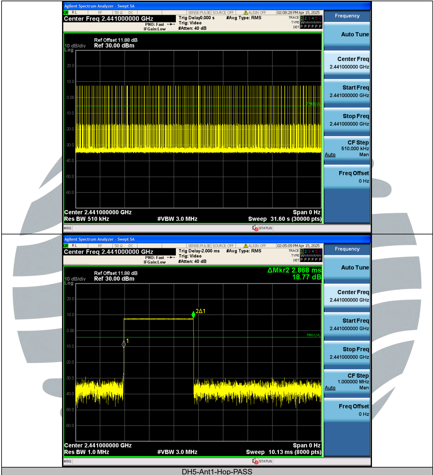
DH5-Ant1-Hop-PASS
