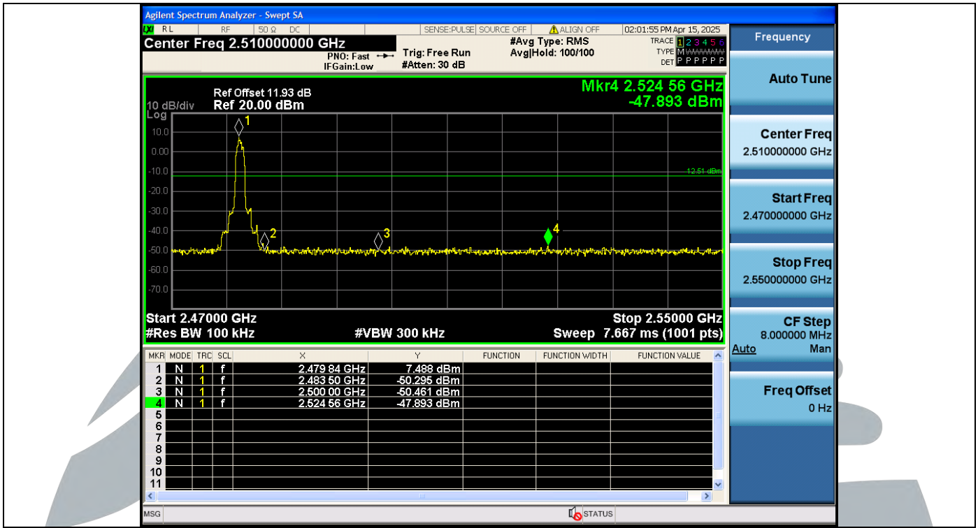
3DH5-Ant1-2480 MHz-PASS
