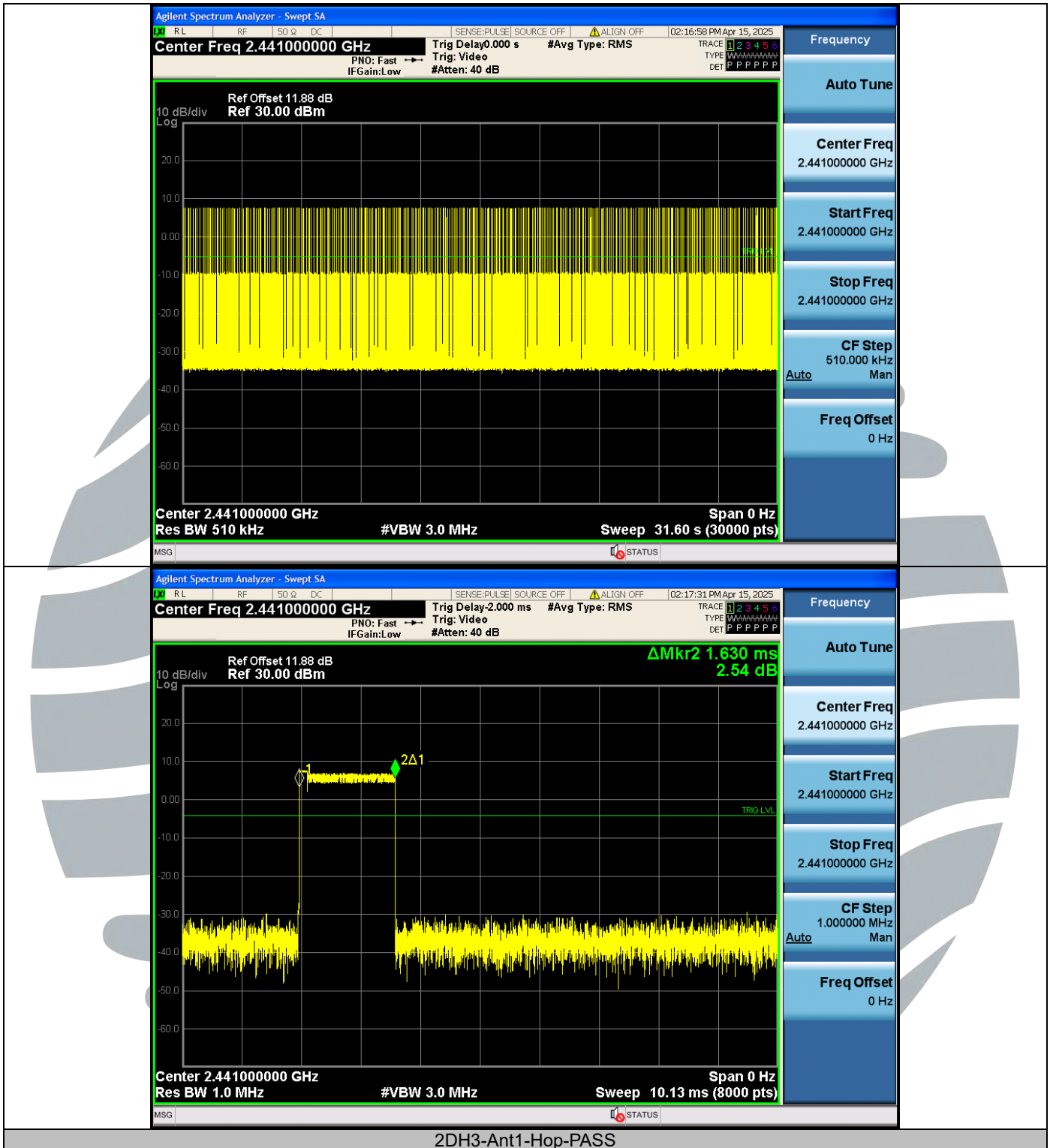
2DH3-Ant1-Hop-PASS
