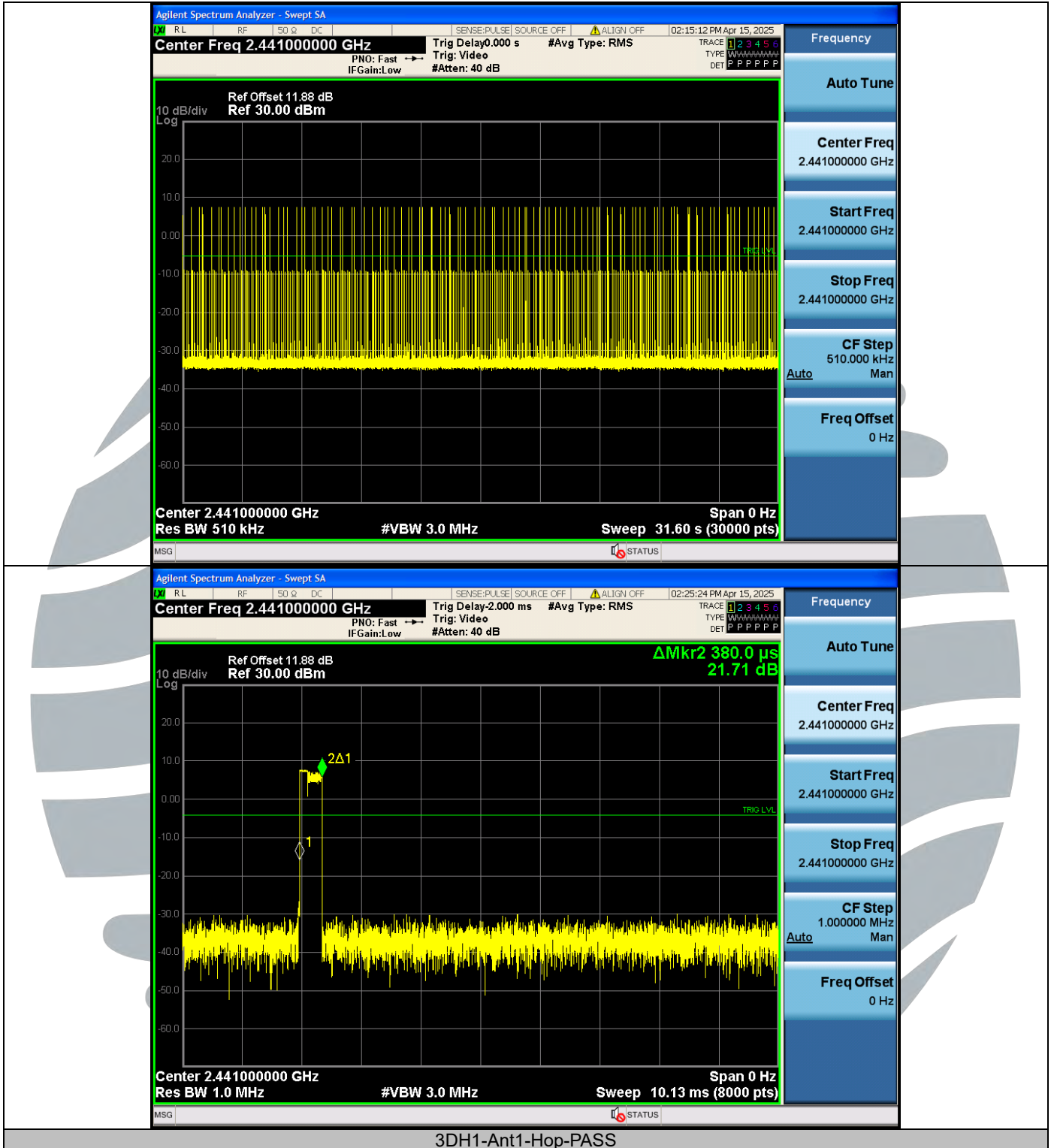
3DH1-Ant1-Hop-PASS
