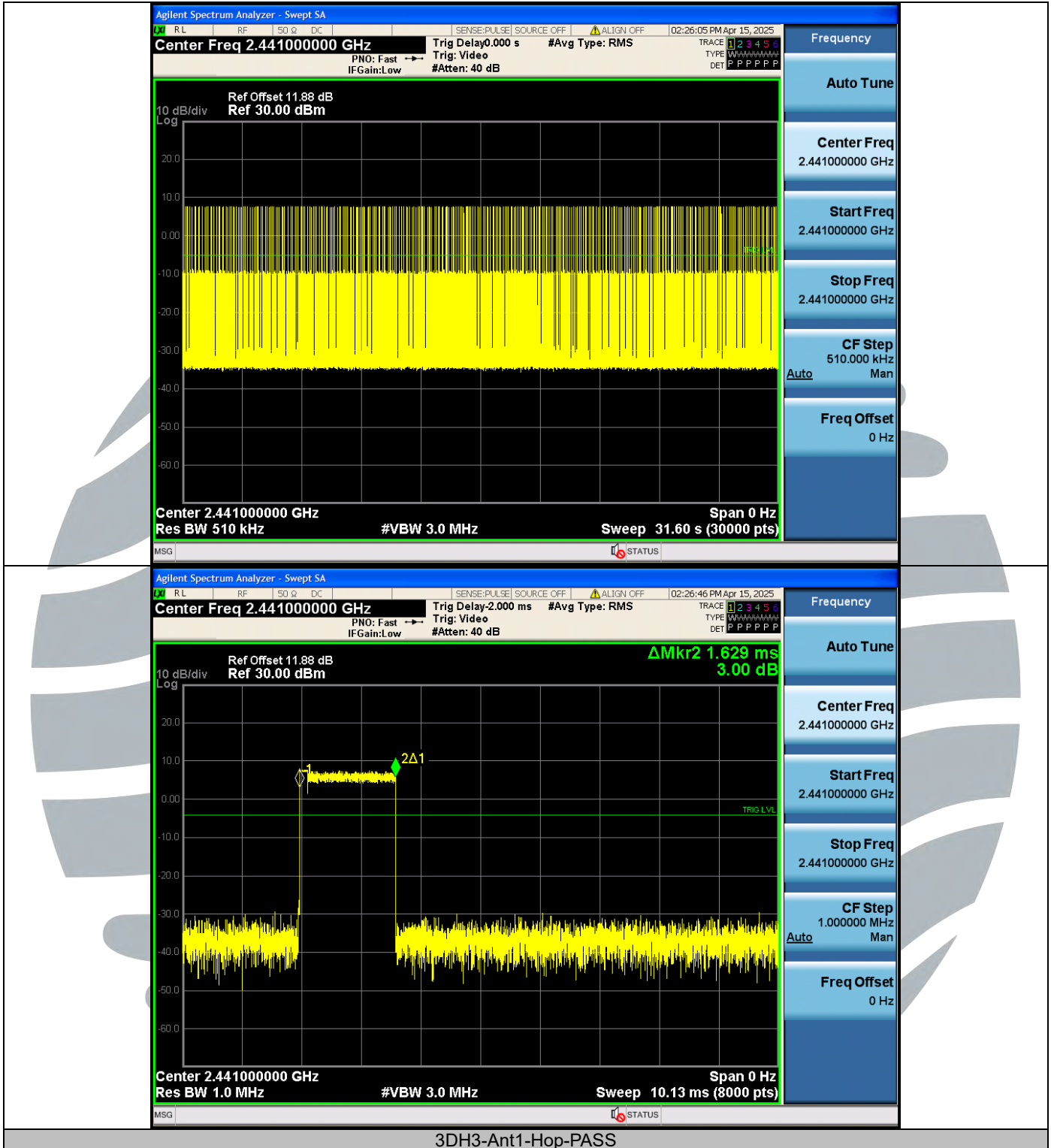
3DH3-Ant1-Hop-PASS
