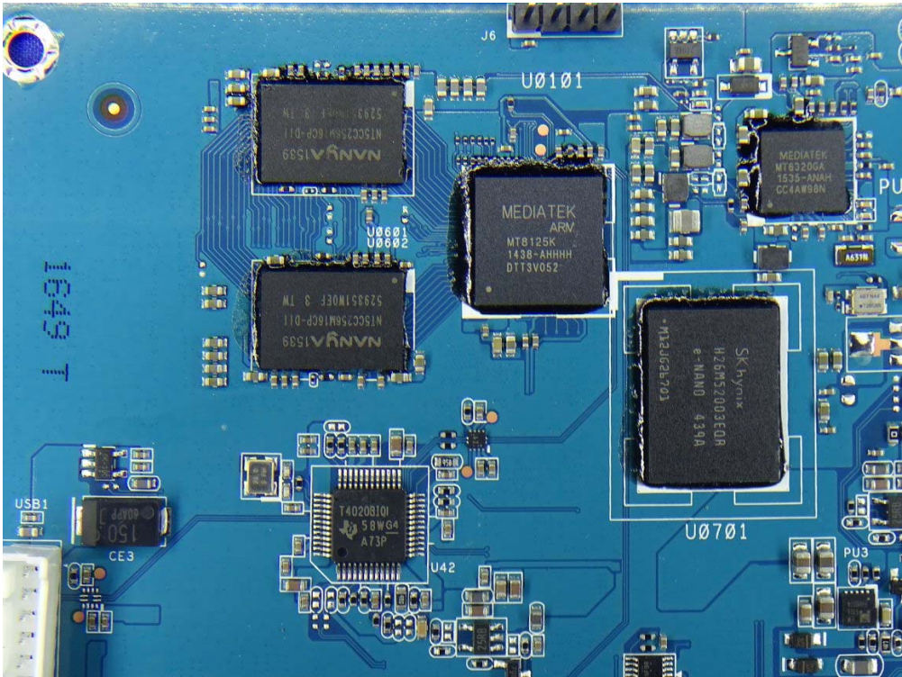
(26) EUT Photo
