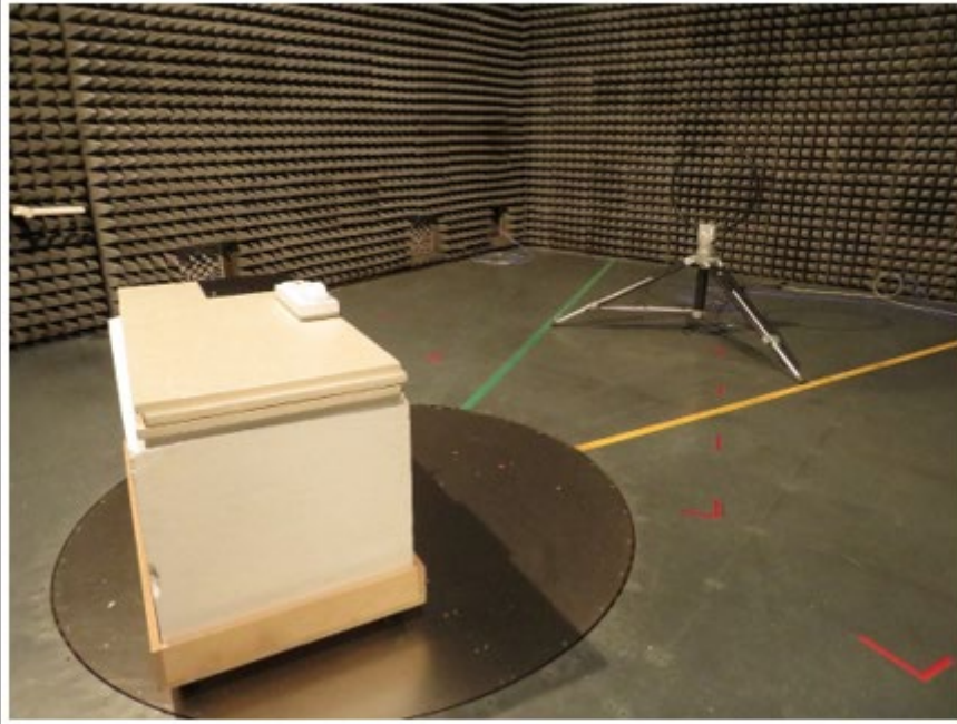
Test setup below 30 MHz - view 1
