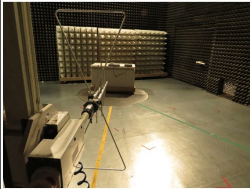
Test setup above 30 MHz - view 2
