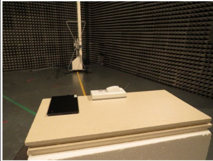
Test setup above 30 MHz - view 1
