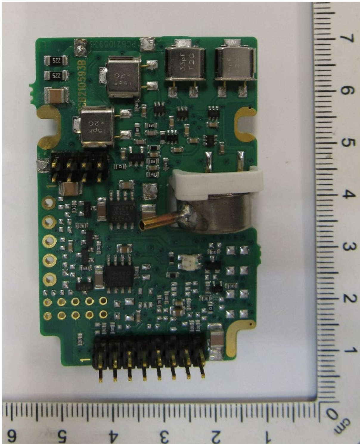
Barometer module unshielded down view
