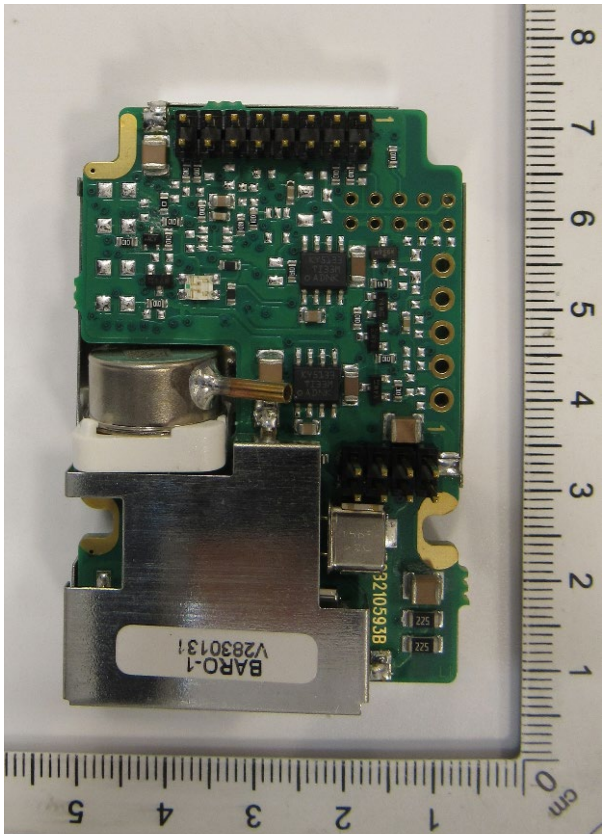
Barometer module down view
