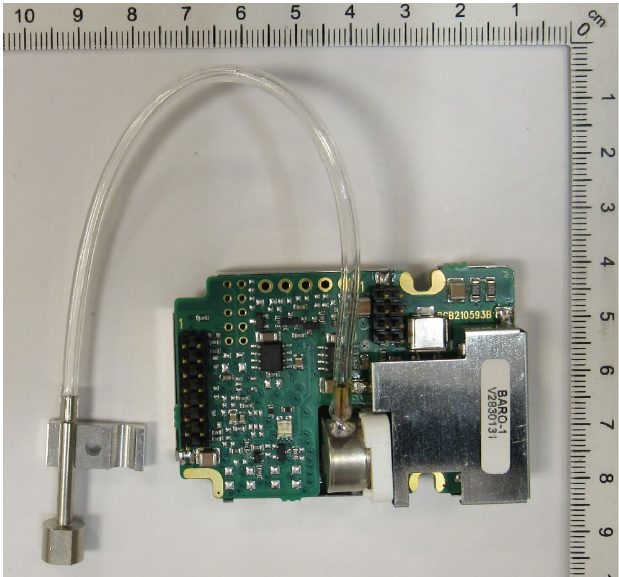
Barometer module with host
