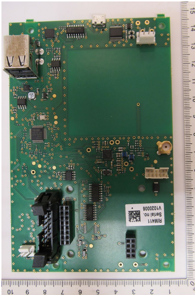
EUT Front PCB
