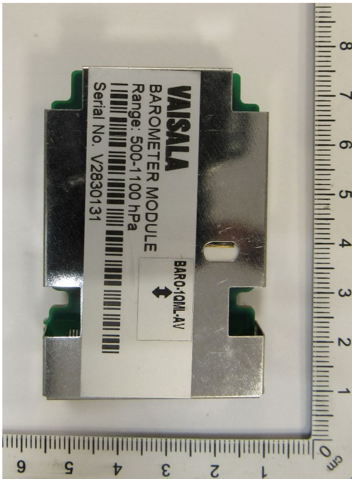
Barometer module top view
