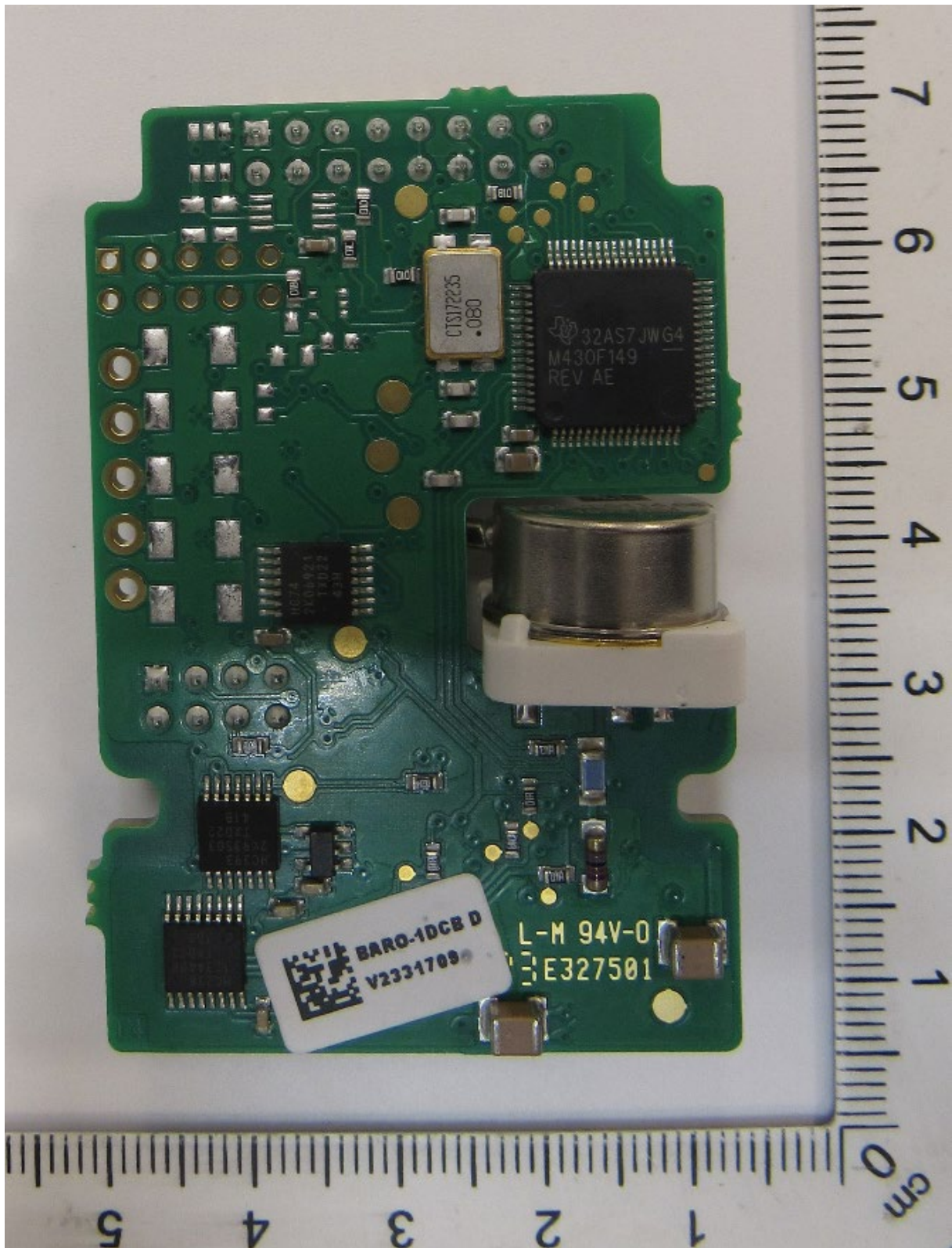
Barometer module unshielded top view
