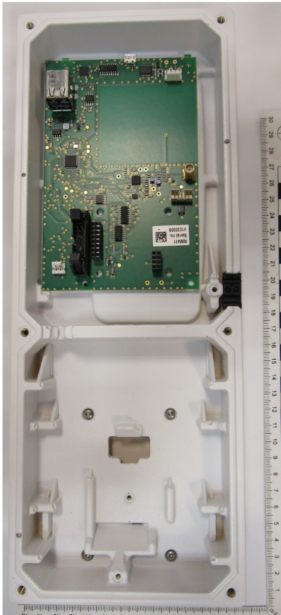
EUT internal view w.o barometer module
