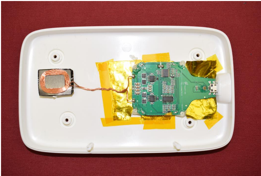
Picture 3: Power transmitter – Open, bottom side, without additional modification copper foil
