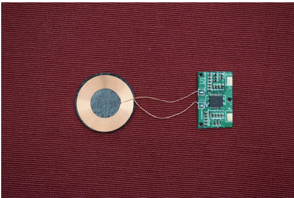
Picture 6: Peripheral device - Power Receiver – PCB, top side
