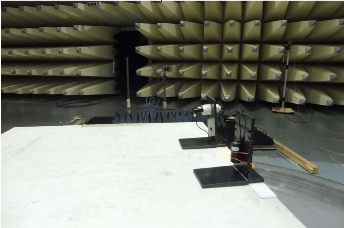
Photo 3: test setup of conducted emission
