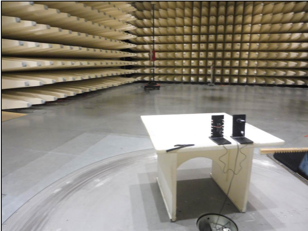
Photo 2: radiated emission set 1
