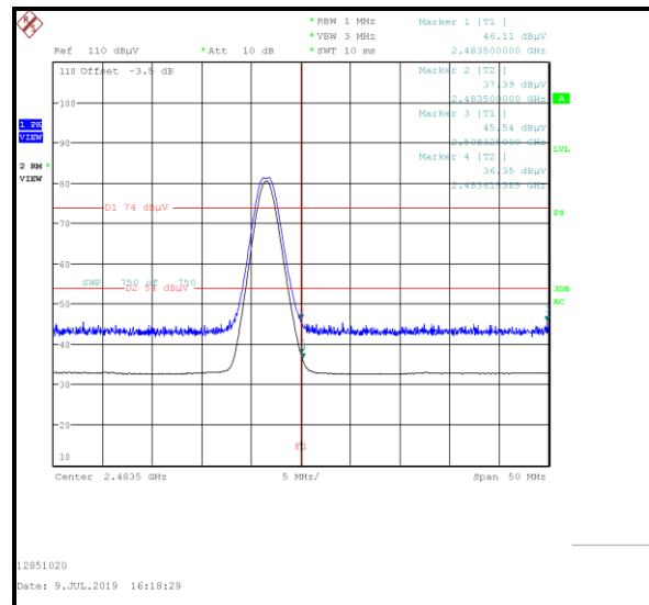
Upper Band Edge Peak and Average Measurement
