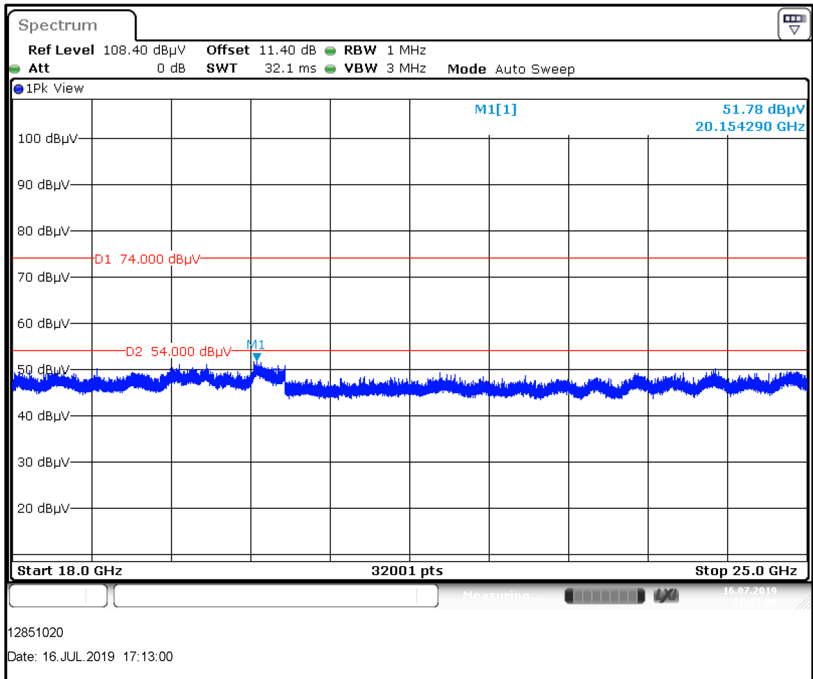
Plot:18 GHz-25 GHz: Bluetooth Low Energy / Bottom Channel
