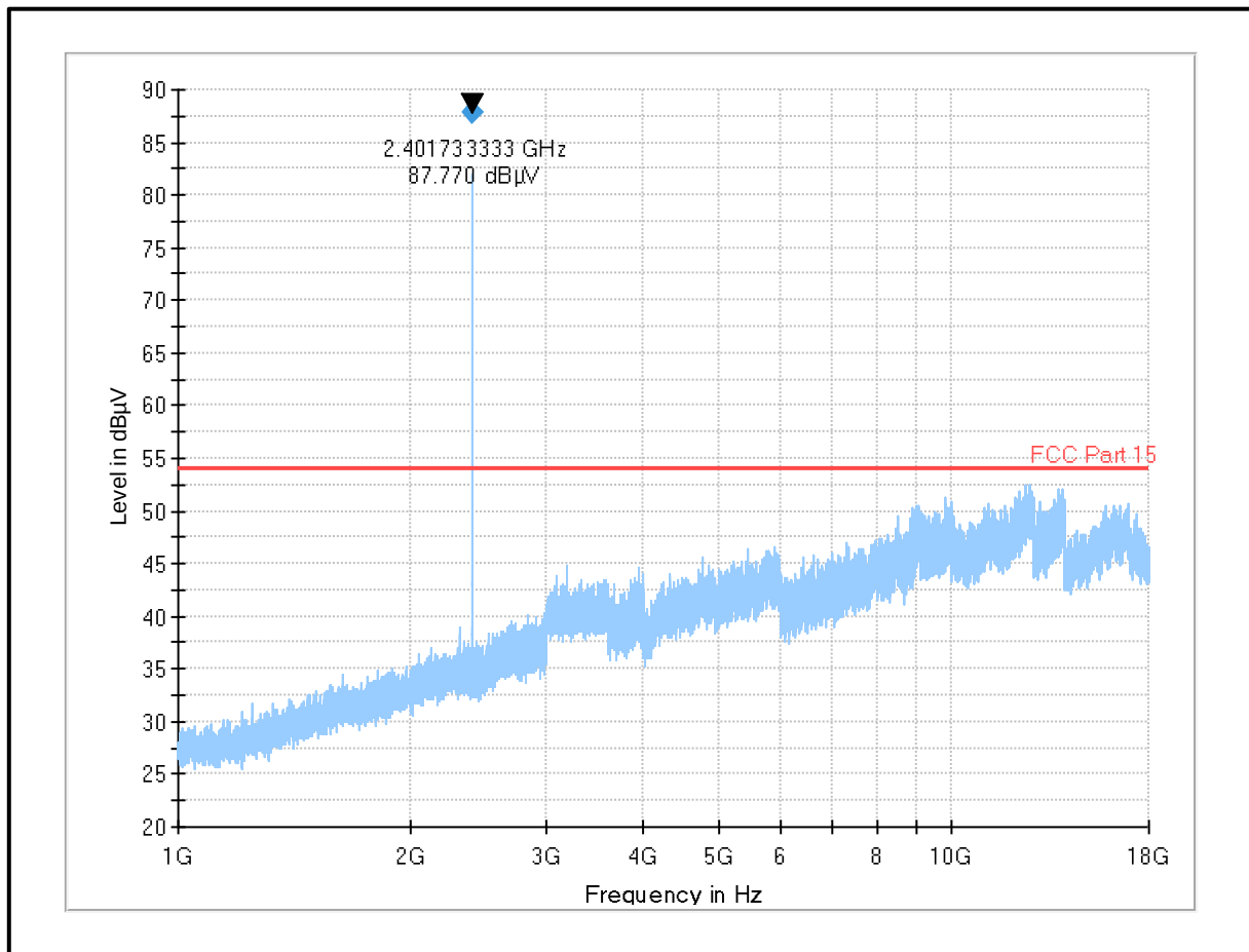
Plot:1 GHz-18 GHz: Bluetooth Low Energy / Bottom Channel
