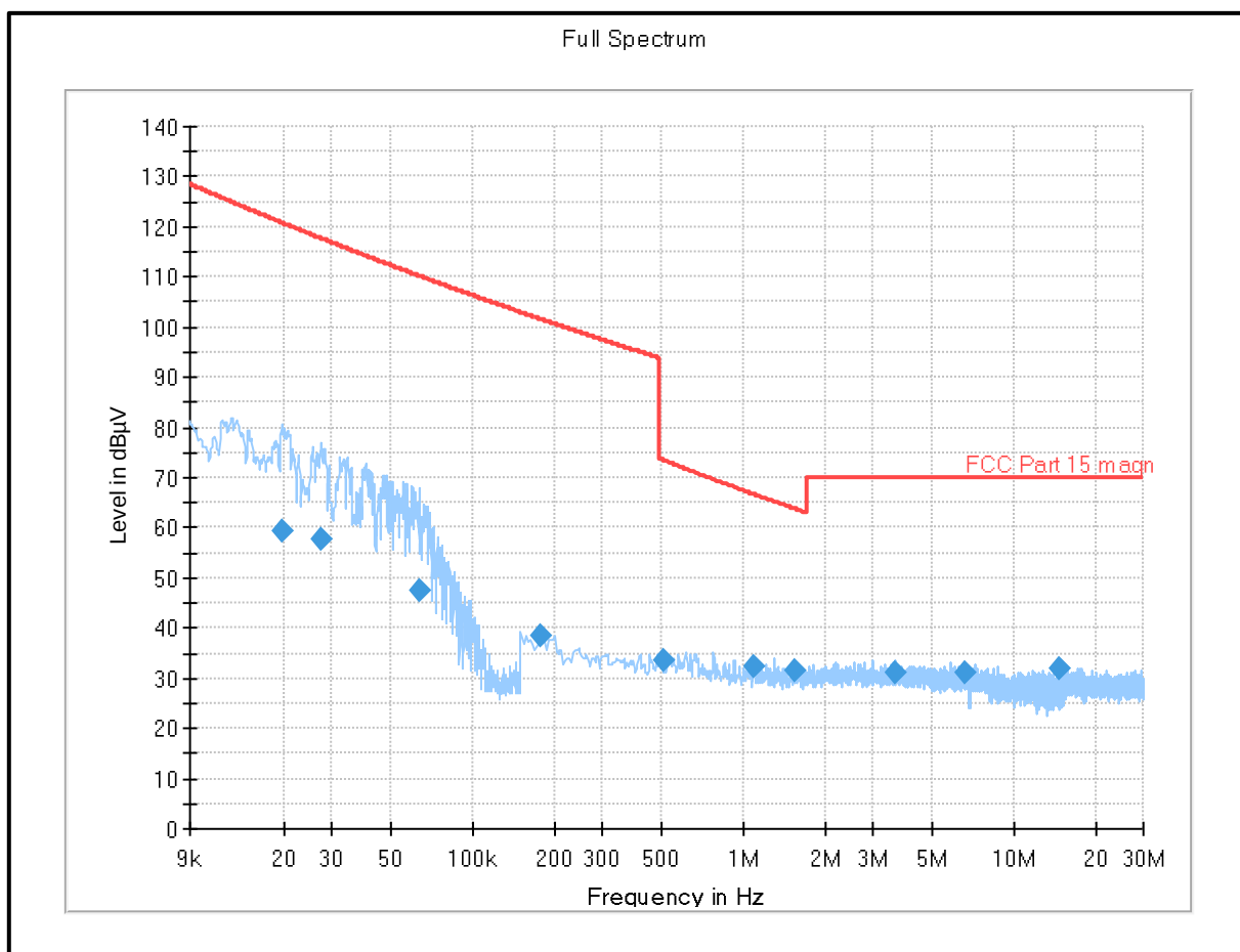
Plot: 9 kHz – 30 MHz: Bluetooth Low Energy / Bottom Channel
