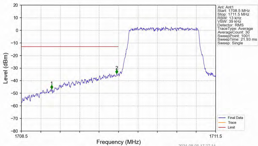
Band66_1.4MHz_16QAM_LCH_1710.7MHz_RB_6_0_NTNV
