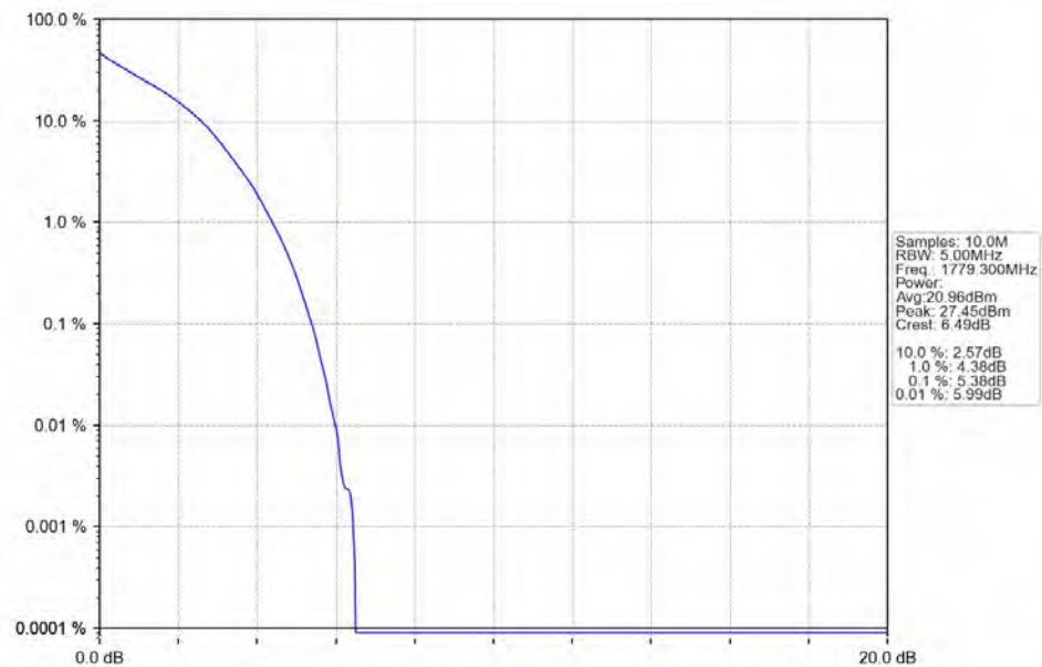
Band66_1.4MHz_QPSK_HCH_1779.3MHz_RB_6_0_NTNV
