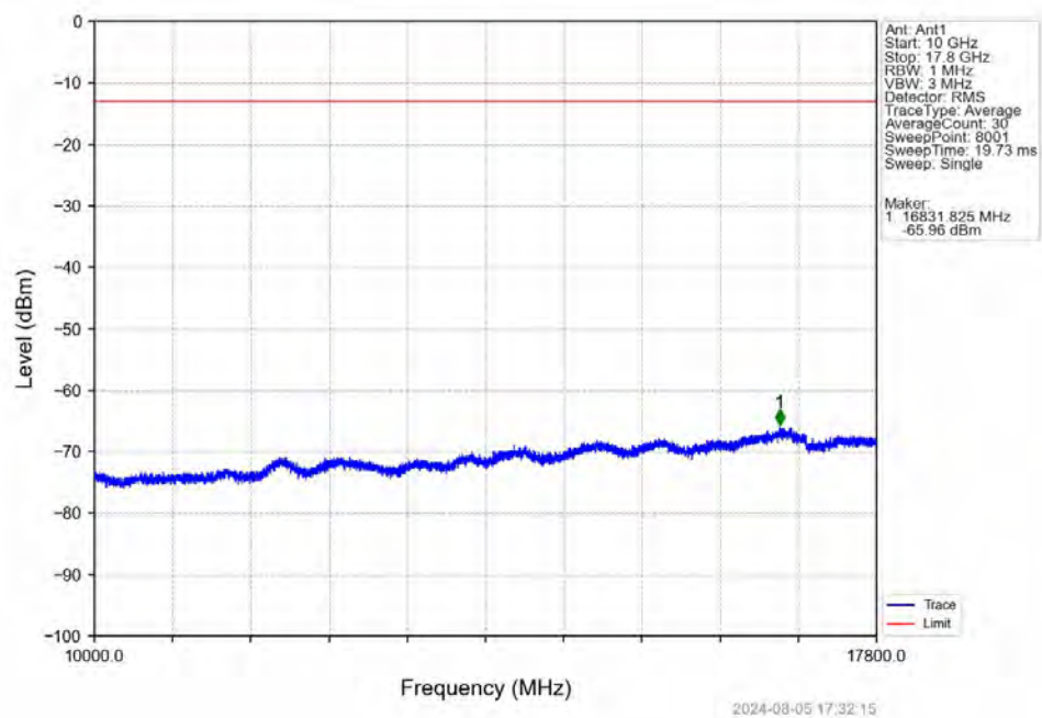
Band66_3MHz_16QAM_MCH_1745MHz_RB_1_0_NTNV
