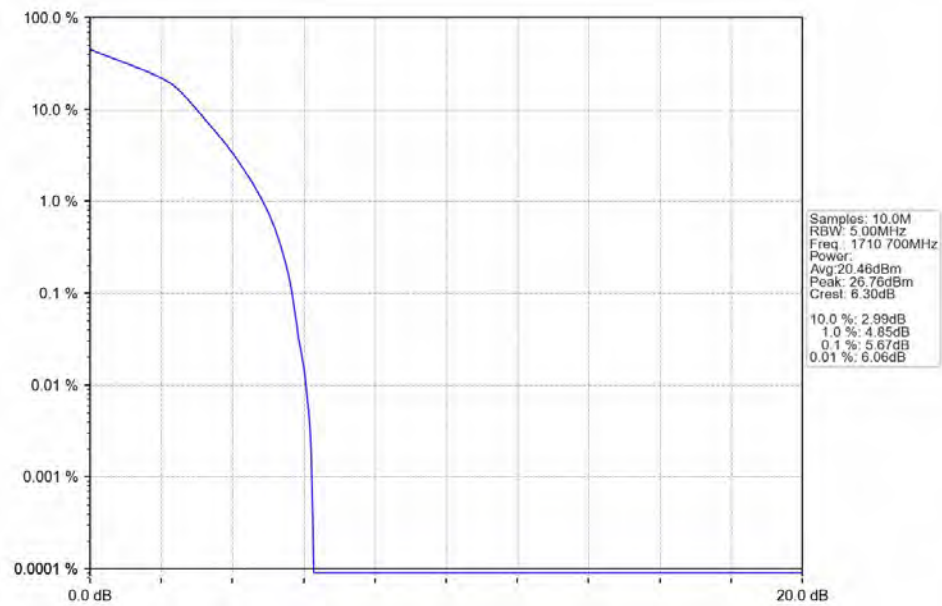
Band66_1.4MHz_16QAM_LCH_1710.7MHz_RB_6_0_NTNV
