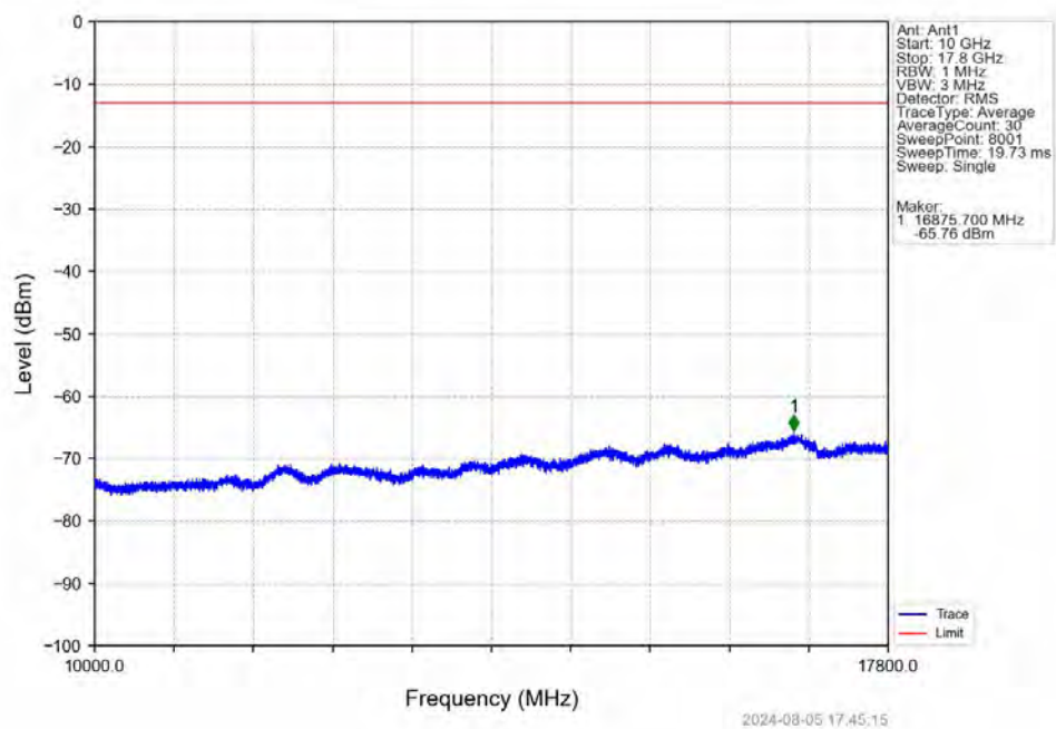
Band66_10MHz_QPSK_HCH_1775MHz_RB_1_0_NTNV
