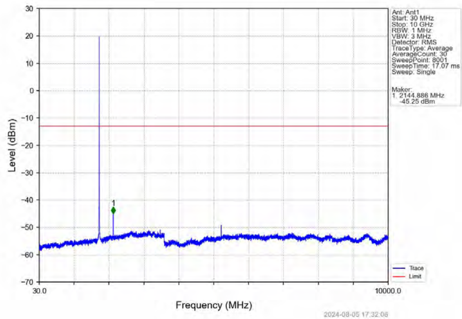
Band66_3MHz_16QAM_MCH_1745MHz_RB_1_0_NTNV
