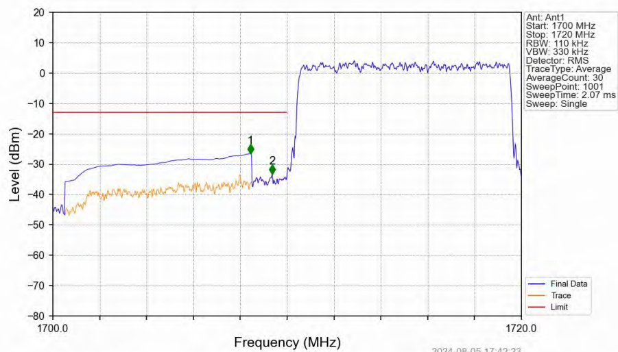
Band66_10MHz_QPSK_LCH_1715MHz_RB_50_0_NTNV
