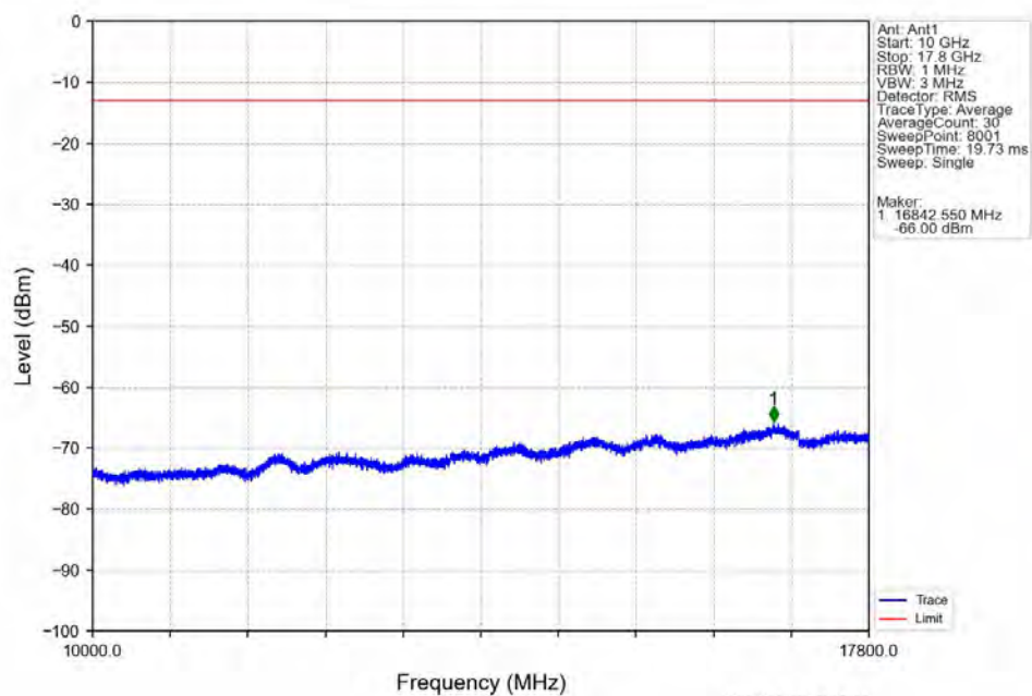
Band66_5MHz_QPSK_HCH_1777.5MHz_RB_1_0_NTNV
