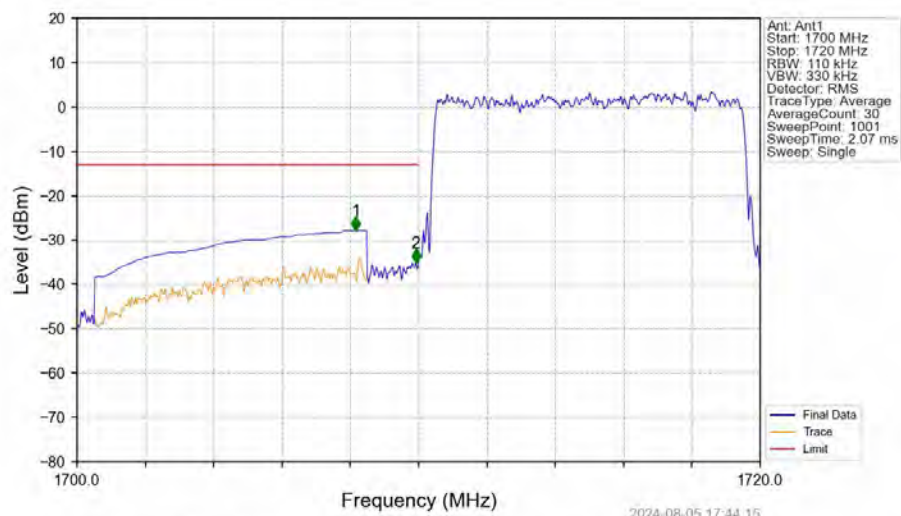
Band66_10MHz_16QAM_LCH_1715MHz_RB_50_0_NTNV
