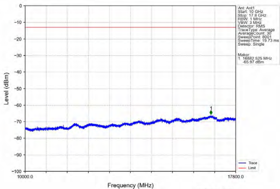
Band66_1.4MHz_16QAM_MCH_1745MHz_RB_1_0_NTNV
