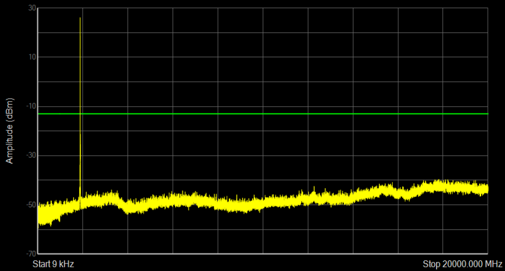
Band25 16QAM BW=15MHz Channel=26615 RB Size=1 Position=#0
