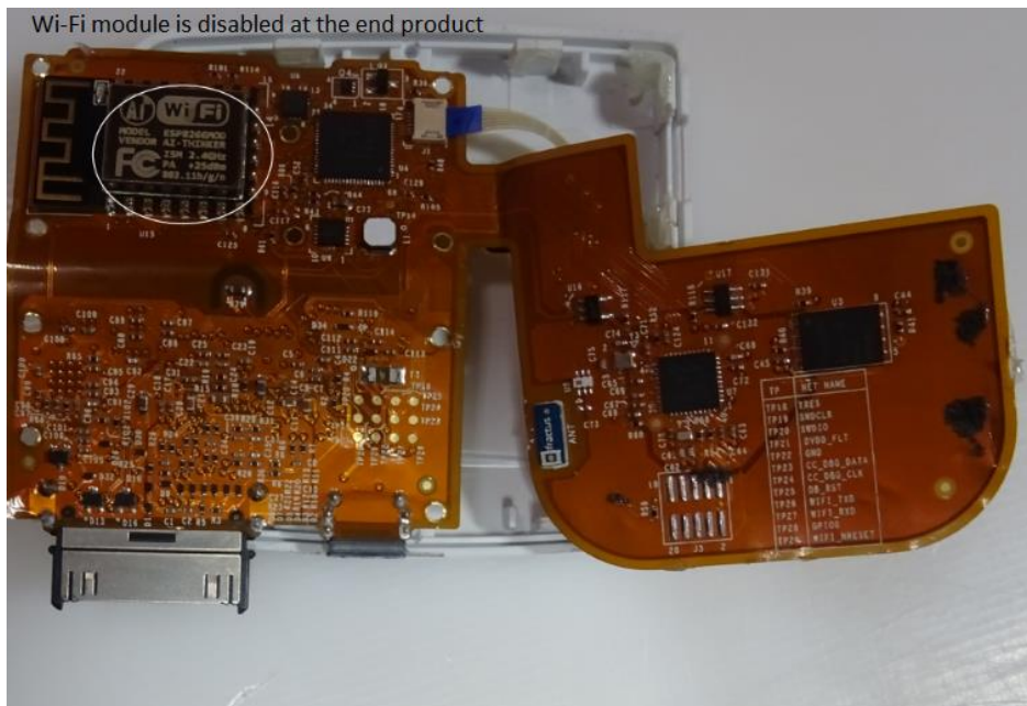
Internal PCB Top view
