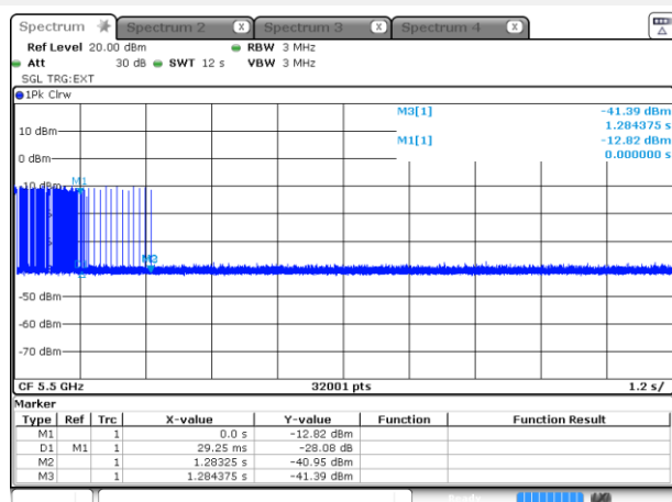
11a Channel 100
