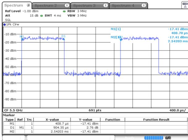
11a-5500 MHz
