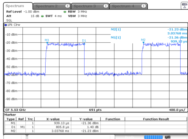
11ac(VHT80)-5530 MHz
