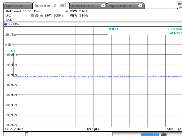
11a Channel 140
