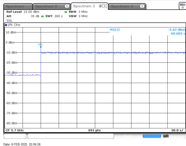
11a-5700 MHz
