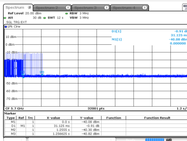
11a Channel 140
