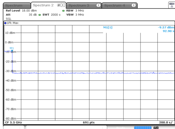
11a Channel 100
