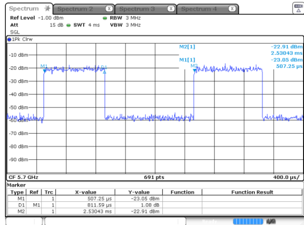
11a-5700 MHz
