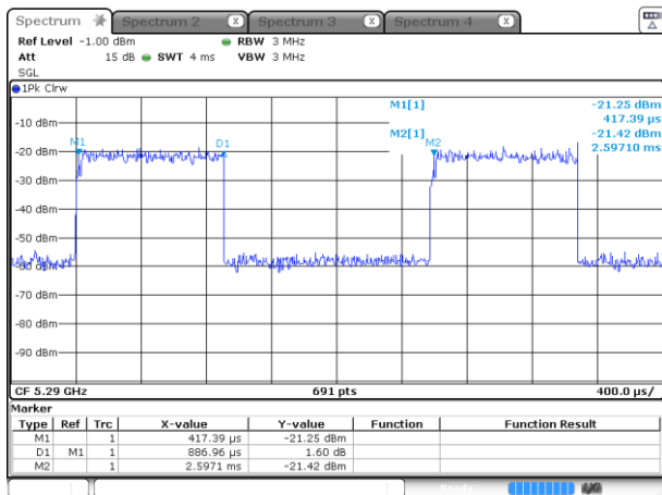
11ac(VHT80)-5290 MHz
