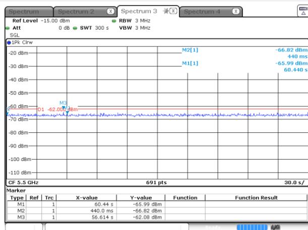
11a-5500 MHz
