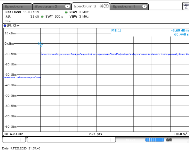
11a-5500 MHz
