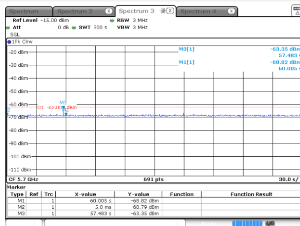
11a-5700 MHz
