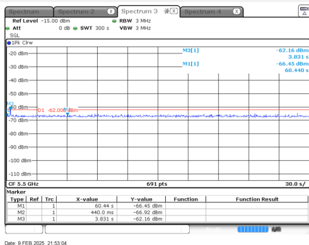
11a-5500 MHz
