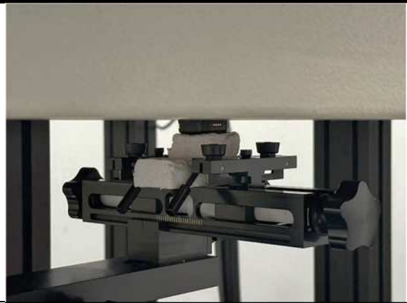
Rear Face of EUT with 0cm Gap
