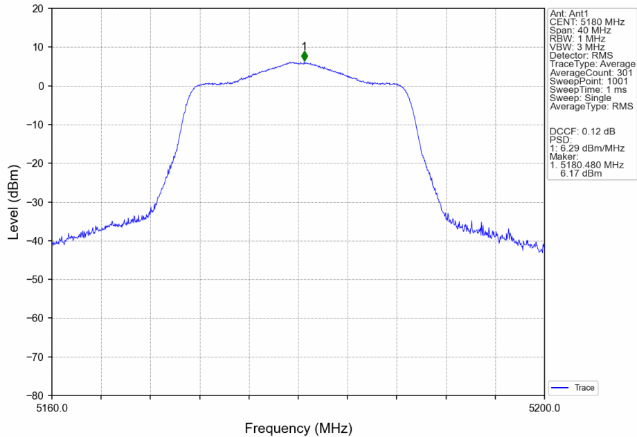
802.11ax(HEW20)_LCH_5180MHz_SU_MIMO_NTNV
