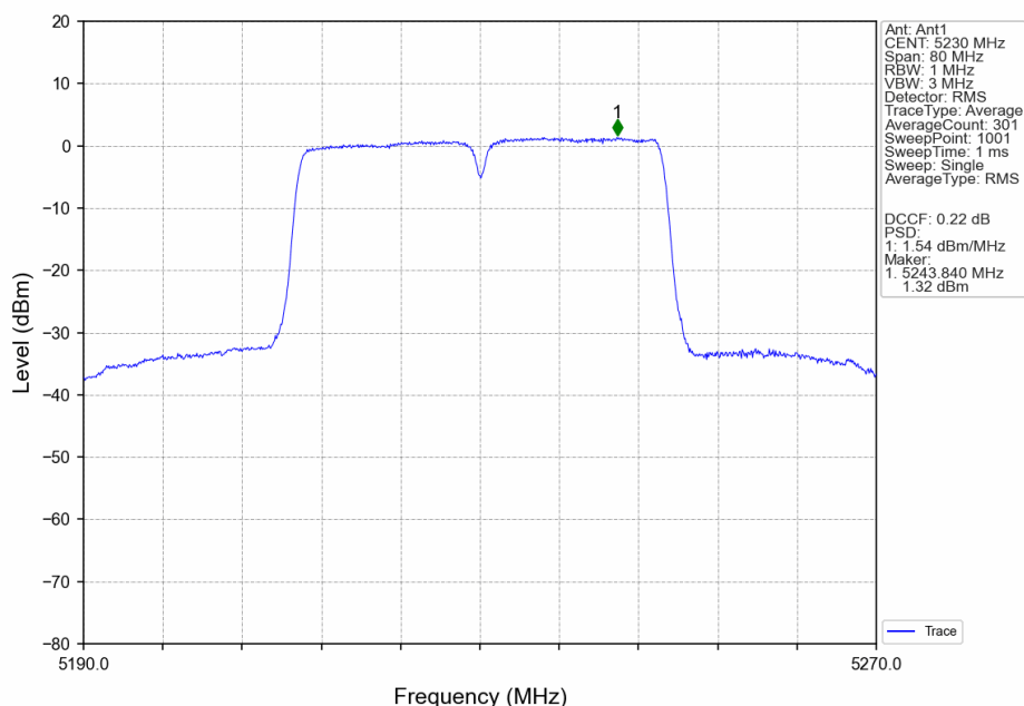
802.11ax(HEW40)_HCH_5230MHz_SU_MIMO_NTNV
