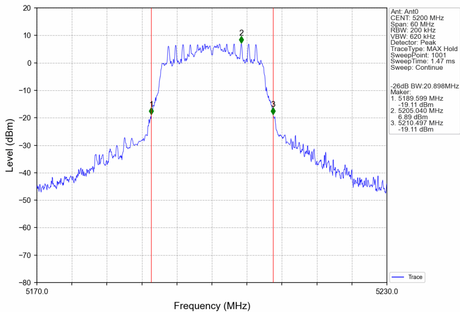
802.11ax(HEW20)_MCH_5200MHz_SU_Ant0_NTNV
