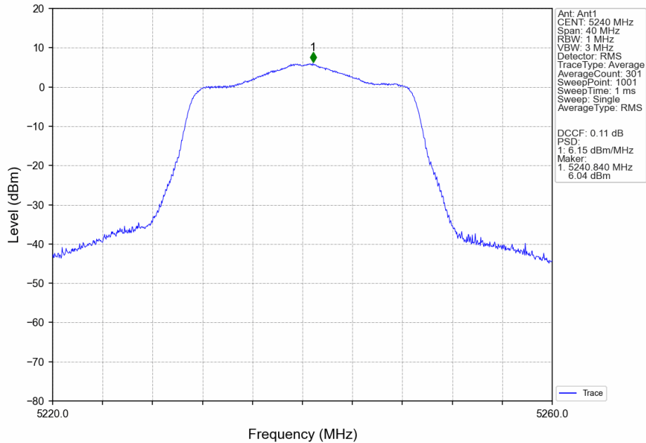
802.11ax(HEW20)_HCH_5240MHz_SU_MIMO_NTNV
