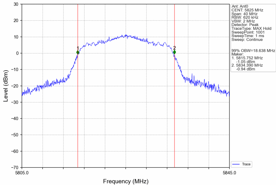
802.11ax(HEW20)_HCH_5825MHz_SU_Ant0_NTNV
