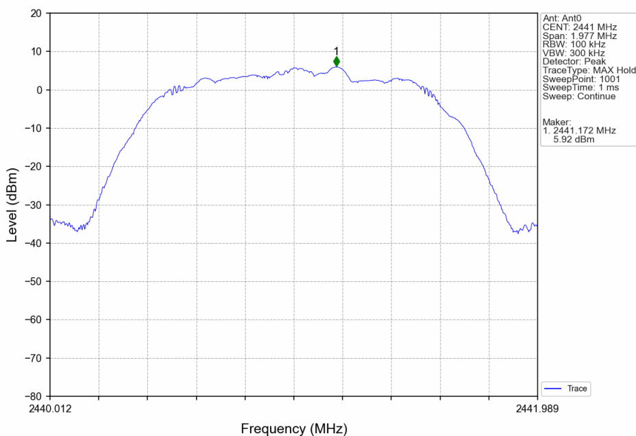
8DPSK_3DH5_MCH_2441MHz_Ant0_NTNV
