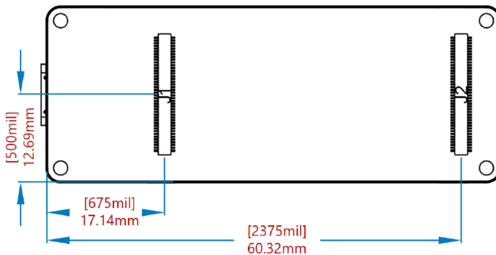
Connectors positions bottom
