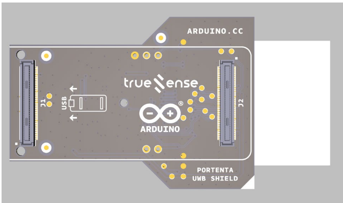
Connectors positions bottom
