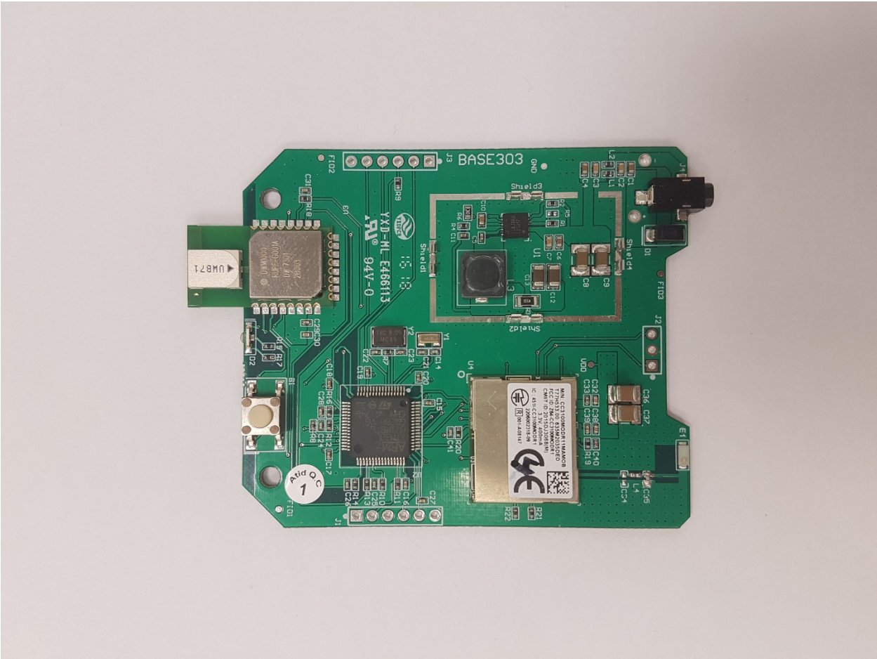
Figure 1: Front View
