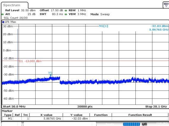
1.4MHz_High_QPSK_1@0(30MHz~20.1GHz)
