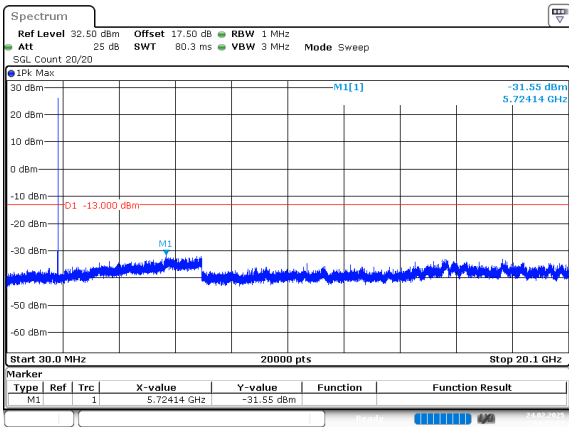
1.4MHz_Low_QPSK_1@0(30MHz~20.1GHz)
